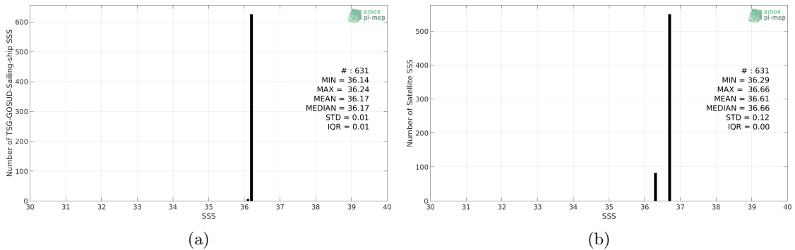
Figure 2: Histograms of SSS from TSG-GOSUD-Sailing-ship (a) and SMOS-L3-CATDS-CPDC-V321-L2Q (b) considering all match-up pairs per bins of 0.1 over the Gulf of Mexico Pi-MEP region and for the full satellite product period.
