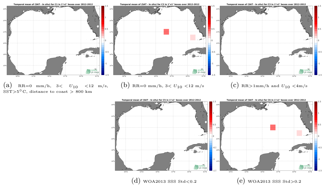
Figure 12: Temporal mean gridded over spatial boxes of size 1^\circ \times 1^\circ of \Delta SSS (SMOS-L3-CATDS-CPDC-V321-L2Q - TSG-GOSUD-Sailing-ship) for 5 different subdatasets corresponding to:RR=0 mm/h, 3 < U_{10} < 12 m/s, SST >5^\circ C, distance to coast > 800 km (a), RR=0 mm/h, 3 < U_{10} < 12 m/s (b), RR >1 mm/h and U_{10} < 4 m/s (c), WOA2013 SSS Std <0.2 (d), WOA2013 SSS Std >0.2 (e).
