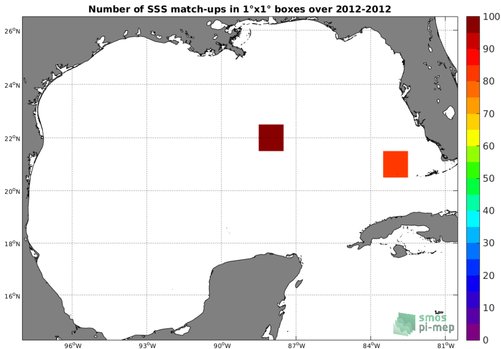
Figure 4: Number of SSS match-ups between TSG-GOSUD-Sailing-ship SSS and the SMOS-L3-CATDS-CPDC-V321-L2Q SSS product for the Gulf of Mexico Pi-MEP region over 1^{\circ} \times 1^{\circ} boxes and for the full satellite product period.
