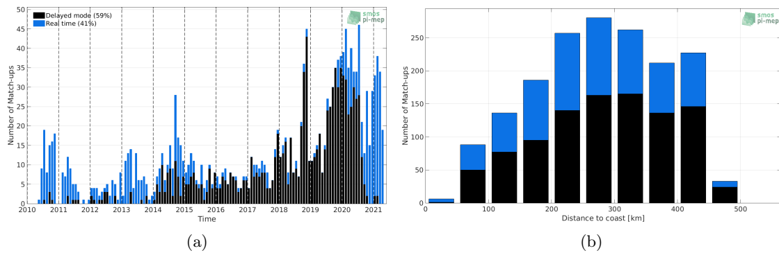
Figure 1: Number of match-ups between Argo and SMOS SSS L2Q v321 - 0.25 Deg (CATDS-CPDC) SSS as a function of time (a) and as function of the distance to coast (b) over the Gulf of Mexico Pi-MEP region and for the full satellite product period.
