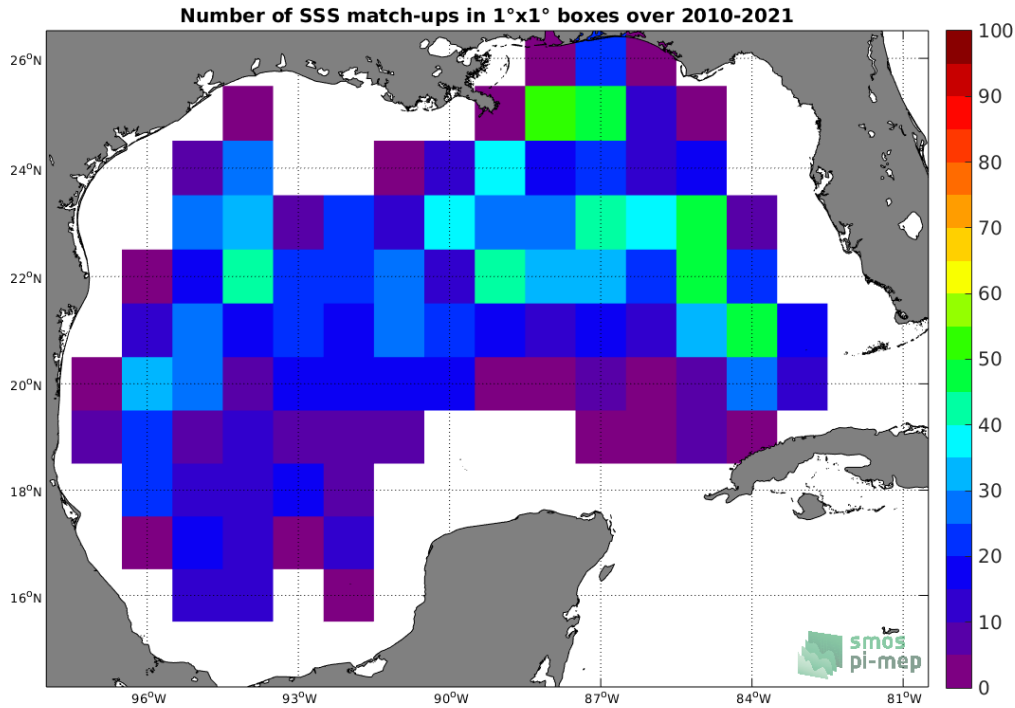
Figure 4: Number of SSS match-ups between Argo SSS and the SMOS SSS L2Q v321 - 0.25 Deg (CATDS-CPDC) SSS product for the Gulf of Mexico Pi-MEP region over 1°x1° boxes and for the full satellite product period.
