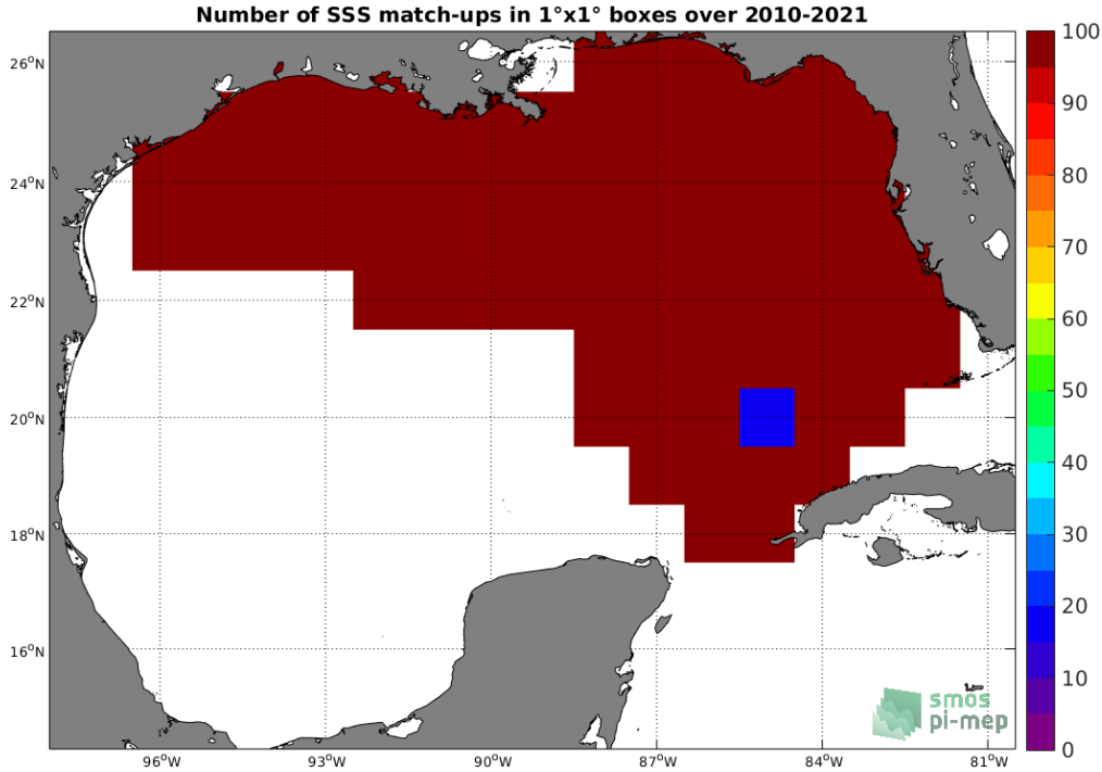
Figure 4: Number of SSS match-ups between TSG (SAMOS) SSS and the SMOS SSS L3 v317 - 10 Days - 25 km (CATDS-CPDC) SSS product for the Gulf of Mexico Pi-MEP region over 1^\circ \times 1^\circ boxes and for the full satellite product period.
