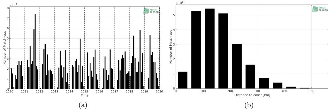
Figure 1: Number of match-ups between TSG-SAMOS and SMOS L3 v317 - 10 Days - 25 km (CATDS-CPDC) SSS as a function of time (a) and as function of the distance to coast (b) over the Gulf of Mexico Pi-MEP region and for the full satellite product period.
