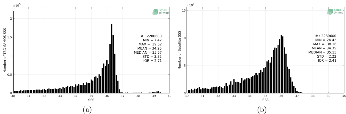
Figure 2: Histograms of SSS from TSG-SAMOS (a) and SMOS L3 v317 - 10 Days - 25 km (CATDS-CPDC) (b) considering all match-up pairs per bins of 0.1 over the Gulf of Mexico Pi-MEP region and for the full satellite product period.
