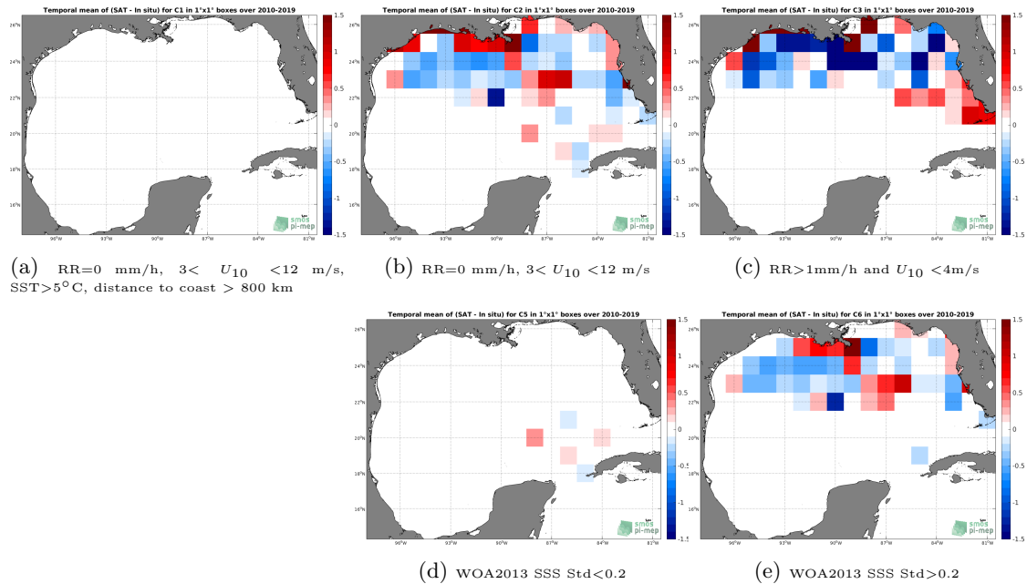
Figure 12: Temporal mean gridded over spatial boxes of size 1^{\circ}\times 1^{\circ} of \Delta\text{SSS} (SMOS L3 v317 - 10 Days - 25 km (CATDS-CPDC) - TSG-SAMOS) for 5 different subdatasets corresponding to:RR=0 mm/h, 3 < U_{10} < 12 m/s, SST >5^{\circ}\text{C} , distance to coast > 800 km (a), RR=0 mm/h, 3 < U_{10} < 12 m/s (b), RR >1 mm/h and U_{10} < 4 m/s (c), WOA2013 SSS Std <0.2 (d), WOA2013 SSS Std >0.2 (e).
