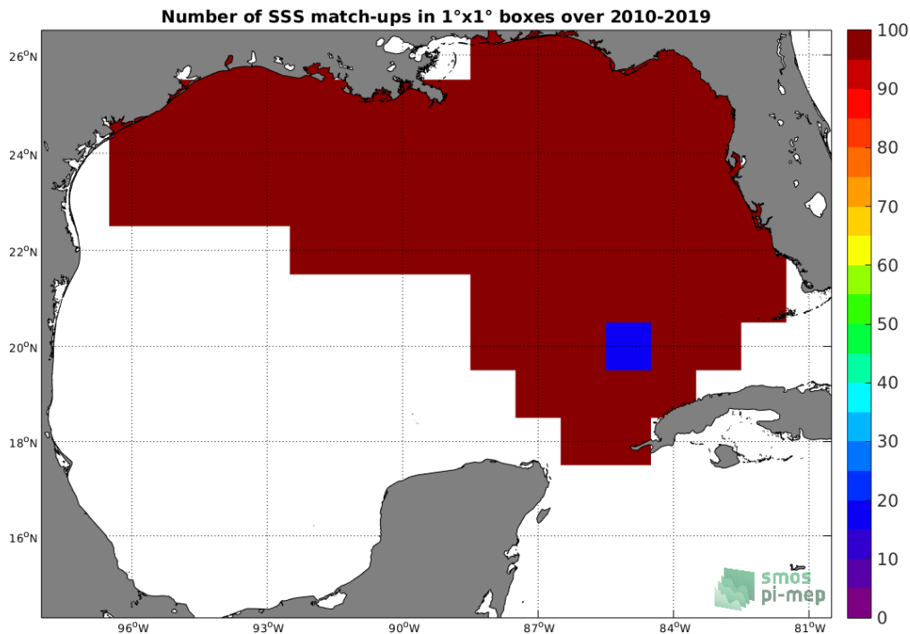
Figure 4: Number of SSS match-ups between TSG-SAMOS SSS and the SMOS L3 v317 - 10 Days - 25 km (CATDS-CPDC) SSS product for the Gulf of Mexico Pi-MEP region over 1°x1° boxes and for the full satellite product period.
