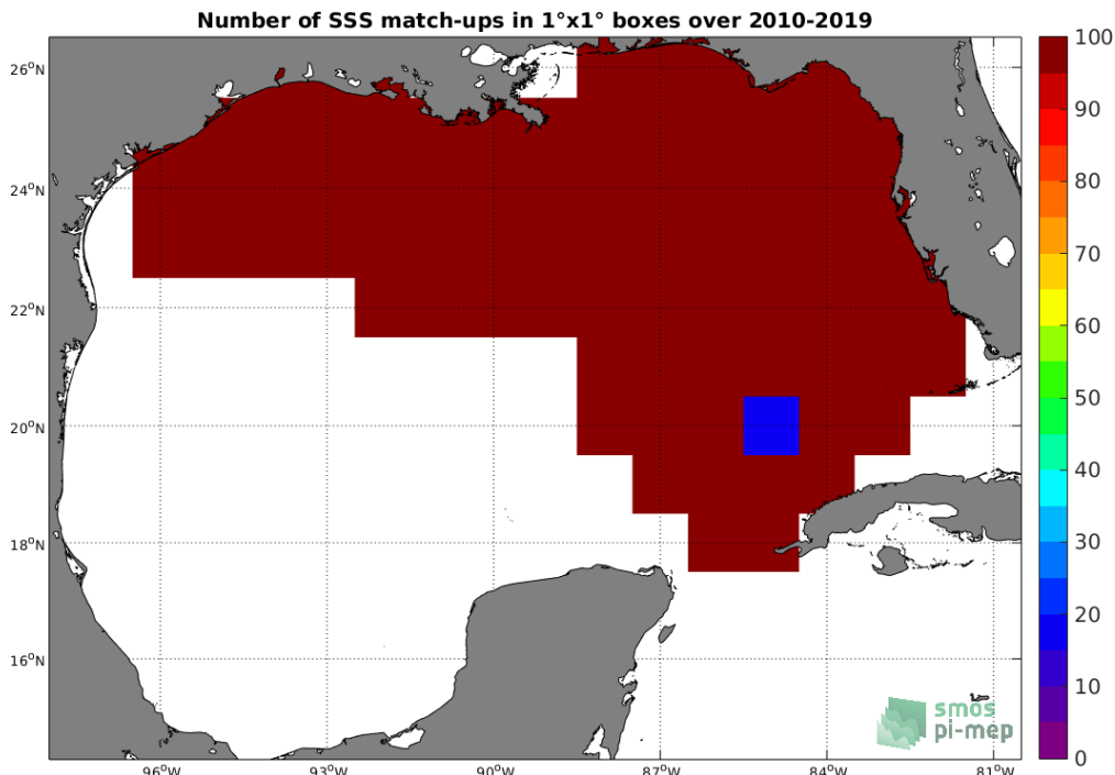
Figure 4: Number of SSS match-ups between TSG-SAMOS SSS and the SMOS-L3-CATDS-CPDC-V317-10DAYS-25KM SSS product for the Gulf of Mexico Pi-MEP region over 1°x1° boxes and for the full satellite product period.
