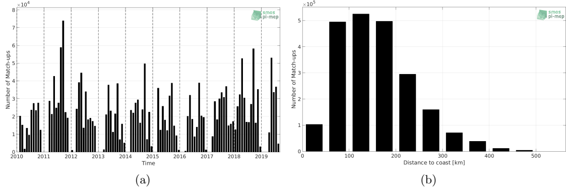
Figure 1: Number of match-ups between TSG-SAMOS and SMOS-L3-CATDS-CPDC-V317-10DAYS-25KM SSS as a function of time (a) and as function of the distance to coast (b) over the Gulf of Mexico Pi-MEP region and for the full satellite product period.
