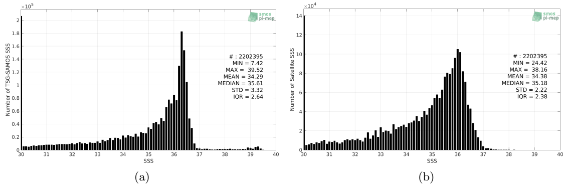
Figure 2: Histograms of SSS from TSG-SAMOS (a) and SMOS-L3-CATDS-CPDC-V317-10DAYS-25KM (b) considering all match-up pairs per bins of 0.1 over the Gulf of Mexico Pi-MEP region and for the full satellite product period.
