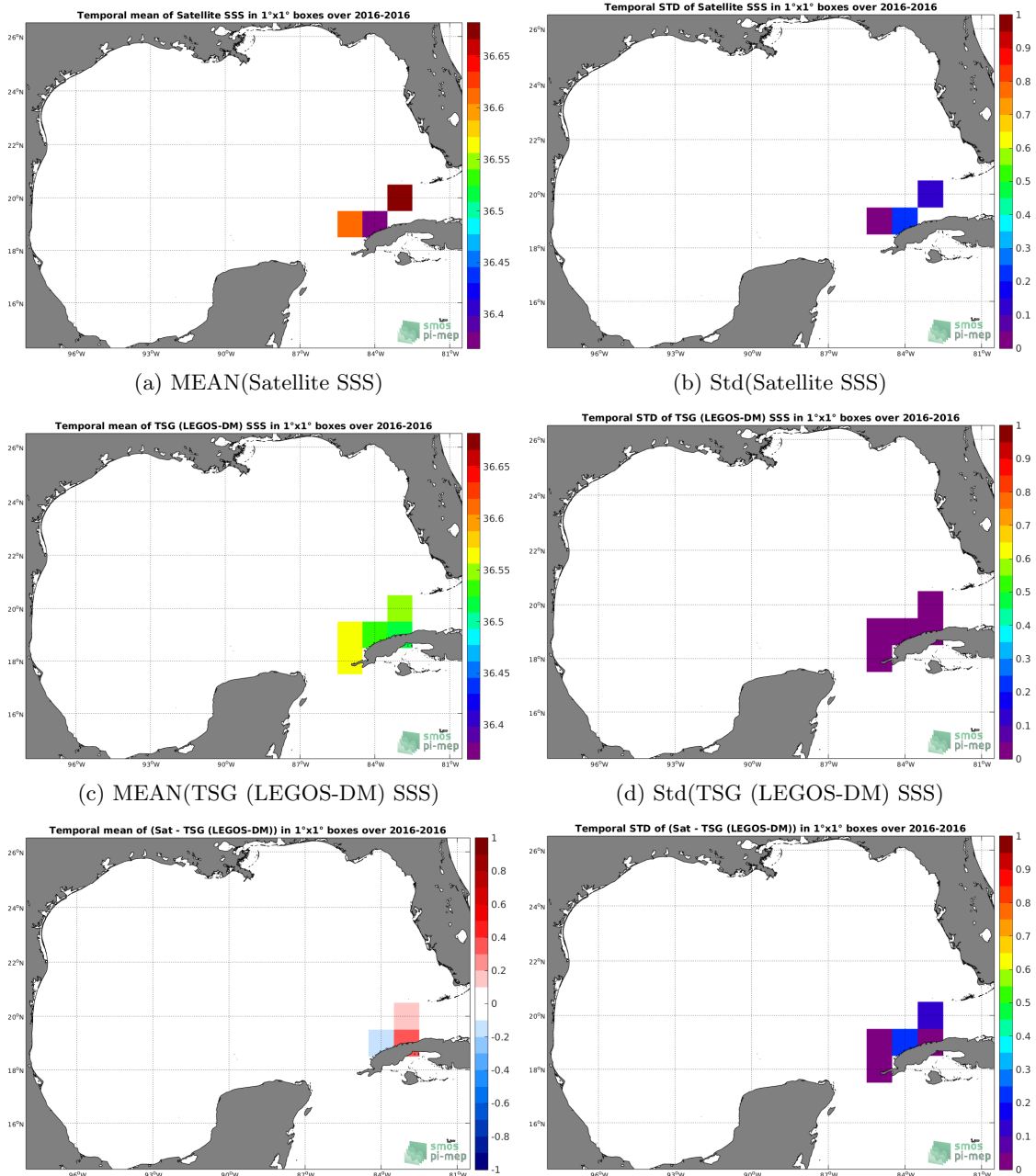
(e) MEAN( \Delta SSS) (Satellite - TSG (LEGOS-DM)) (f) Std( \Delta SSS) (Satellite - TSG (LEGOS-DM)) Figure 6: Temporal mean (left) and Std (right) of SSS from SMOS SSS L3 v317 - 10 Days - 25 km (CATDS-CPDC) (top), TSG (LEGOS-DM) (middle), and of \Delta SSS (Satellite - TSG (LEGOS-DM)). Only match-up pairs are used to generate these maps.
