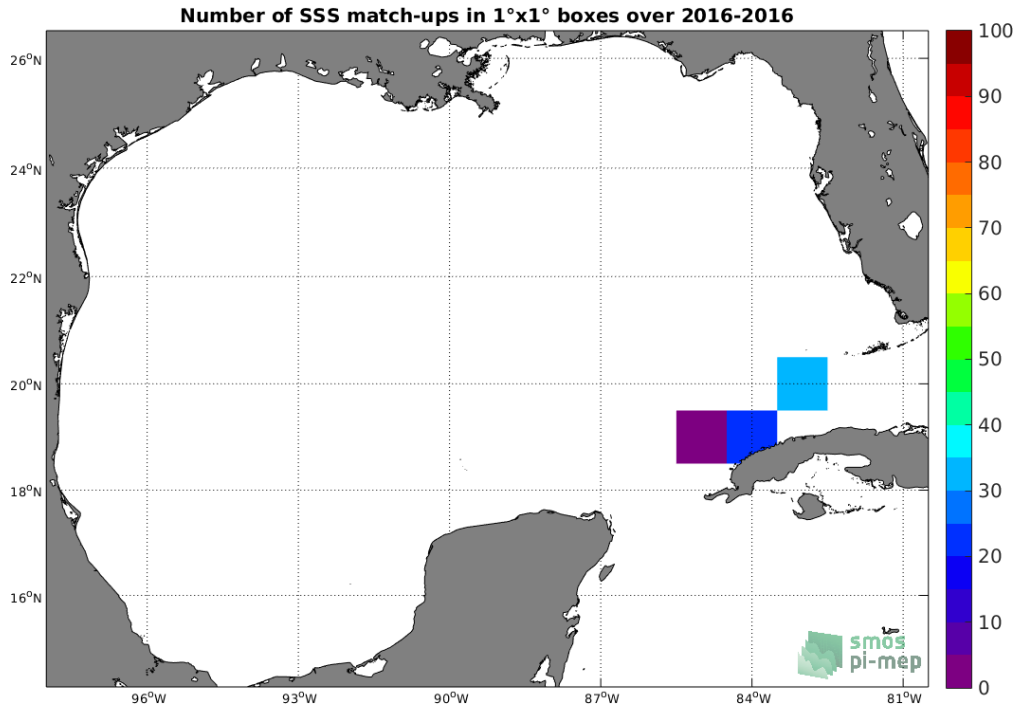
Figure 4: Number of SSS match-ups between TSG (LEGOS-DM) SSS and the SMOS SSS L3 v317 - 10 Days - 25 km (CATDS-CPDC) SSS product for the Gulf of Mexico Pi-MEP region over 1°x1° boxes and for the full satellite product period.
