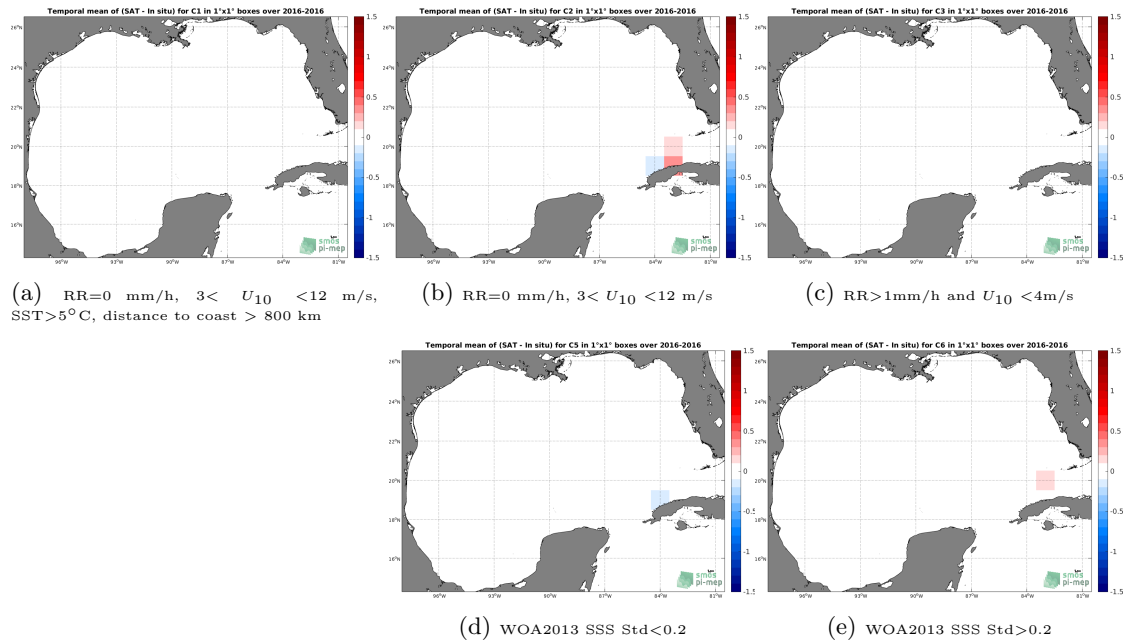
Figure 12: Temporal mean gridded over spatial boxes of size 1^{\circ}\times 1^{\circ} of \Delta\text{SSS} (SMOS L3 v317 - 10 Days - 25 km (CATDS-CPDC) - TSG-LEGOS-DM) for 5 different subdatasets corresponding to:RR=0 mm/h, 3 < U_{10} < 12 m/s, SST >5^{\circ}\text{C} , distance to coast > 800 km (a), RR=0 mm/h, 3 < U_{10} < 12 m/s (b), RR >1 mm/h and U_{10} < 4 m/s (c), WOA2013 SSS Std <0.2 (d), WOA2013 SSS Std >0.2 (e).
