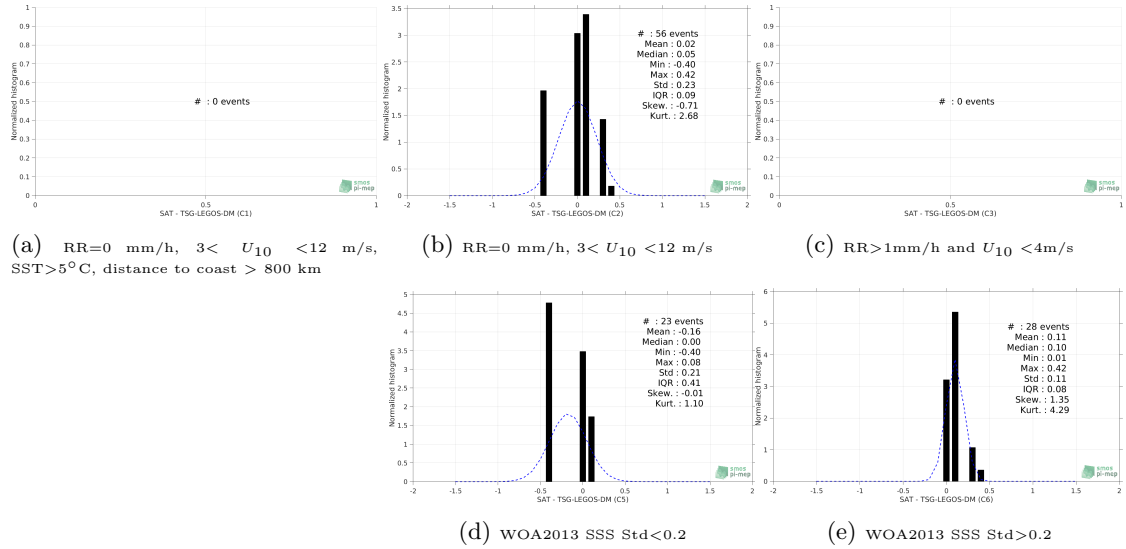
Figure 13: Normalized histogram of \Delta SSS (SMOS L3 v317 - 10 Days - 25 km (CATDS-CPDC) - TSG-LEGOS-DM) for 5 different subdatasets corresponding to: RR=0 mm/h, 3 < U_{10} < 12 m/s, SST > 5°C, distance to coast > 800 km (a), RR=0 mm/h, 3 < U_{10} < 12 m/s (b), RR > 1mm/h and U_{10} < 4 m/s (c), WOA2013 SSS Std < 0.2 (d), WOA2013 SSS Std > 0.2 (e).
