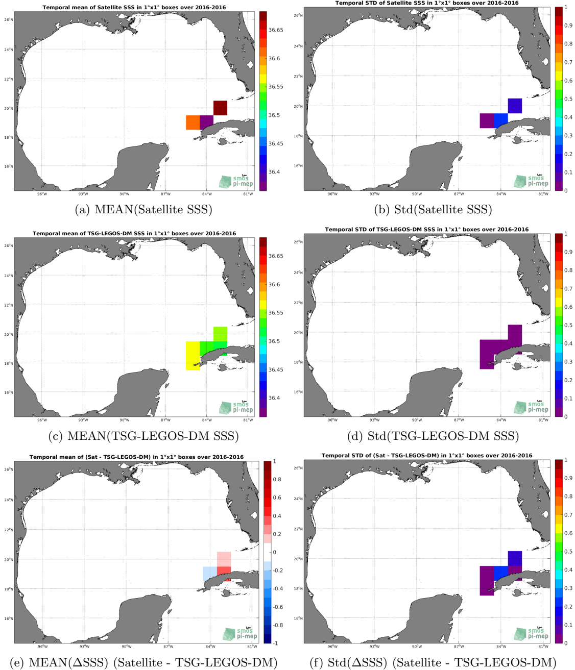
Figure 6: Temporal mean (left) and Std (right) of SSS from SMOS L3 v317 - 10 Days - 25 km (CATDS-CPDC) (top), TSG-LEGOS-DM (middle), and of \Delta SSS (Satellite - TSG-LEGOS-DM). Only match-up pairs are used to generate these maps.
