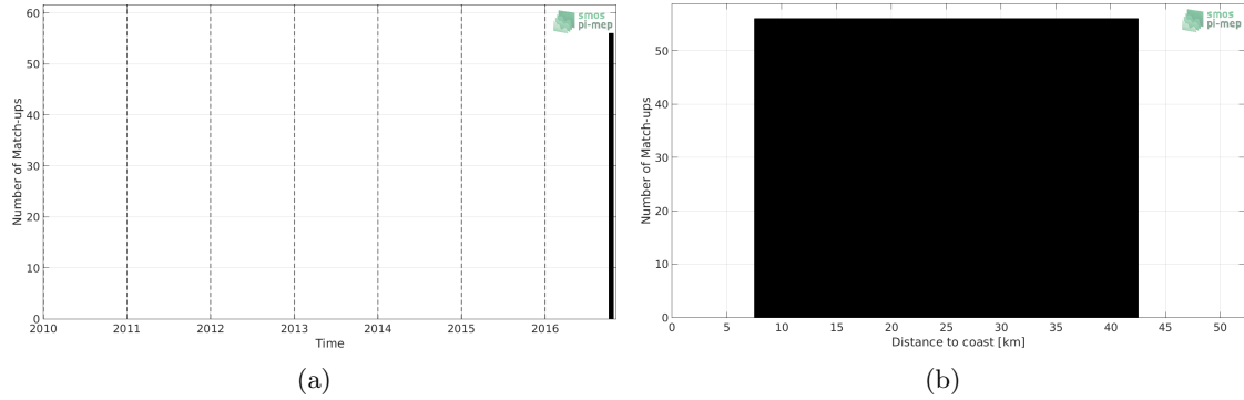
Figure 1: Number of match-ups between TSG-LEGOS-DM and SMOS-L3-CATDS-CPDC-V317-10DAYS-25KM SSS as a function of time (a) and as function of the distance to coast (b) over the Gulf of Mexico Pi-MEP region and for the full satellite product period.
