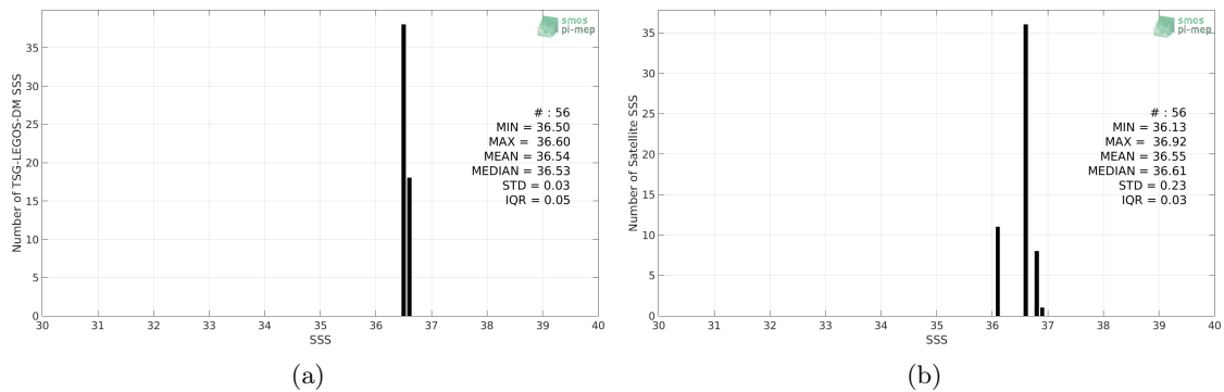
Figure 2: Histograms of SSS from TSG-LEGOS-DM (a) and SMOS-L3-CATDS-CPDC-V317-10DAYS-25KM (b) considering all match-up pairs per bins of 0.1 over the Gulf of Mexico Pi-MEP region and for the full satellite product period.
