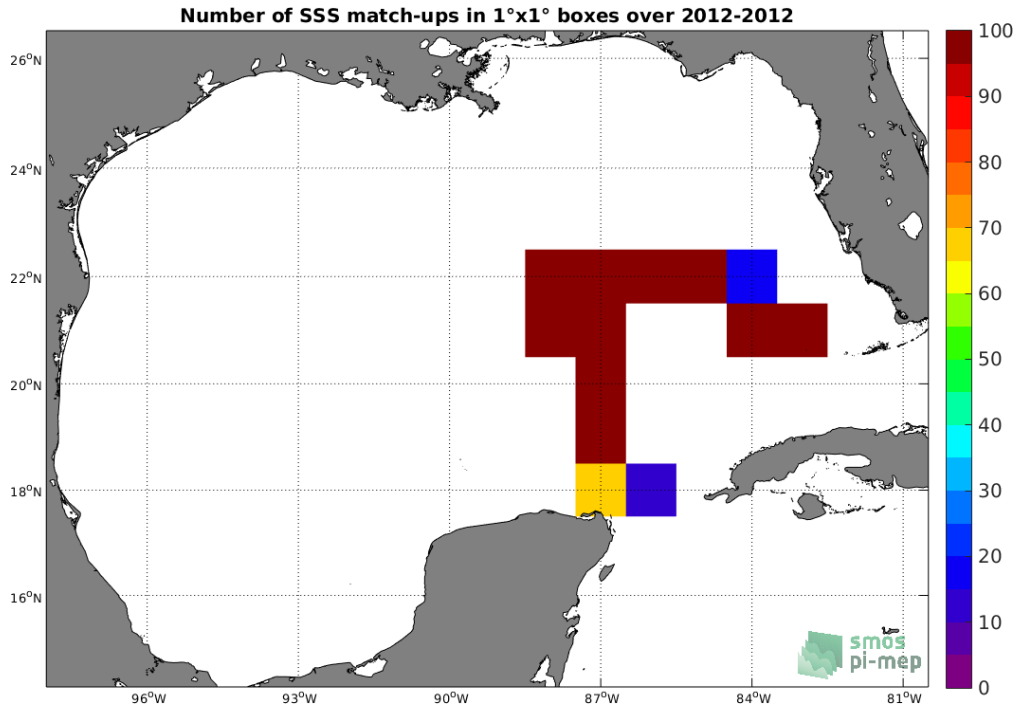
Figure 4: Number of SSS match-ups between TSG (GOSUD-Sailing-ship) SSS and the SMOS SSS L3 v317 - 10 Days - 25 km (CATDS-CPDC) SSS product for the Gulf of Mexico Pi-MEP region over 1°x1° boxes and for the full satellite product period.
