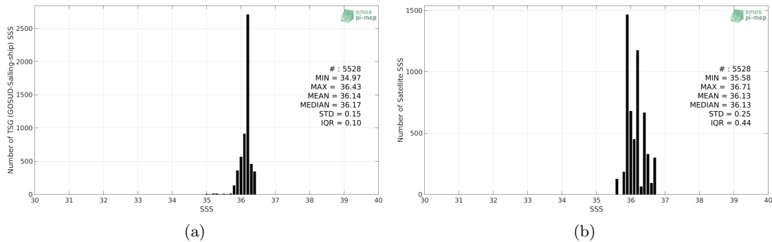
Figure 2: Histograms of SSS from TSG (GOSUD-Sailing-ship) (a) and SMOS SSS L3 v317 - 10 Days - 25 km (CATDS-CPDC) (b) considering all match-up pairs per bins of 0.1 over the Gulf of Mexico Pi-MEP region and for the full satellite product period.
