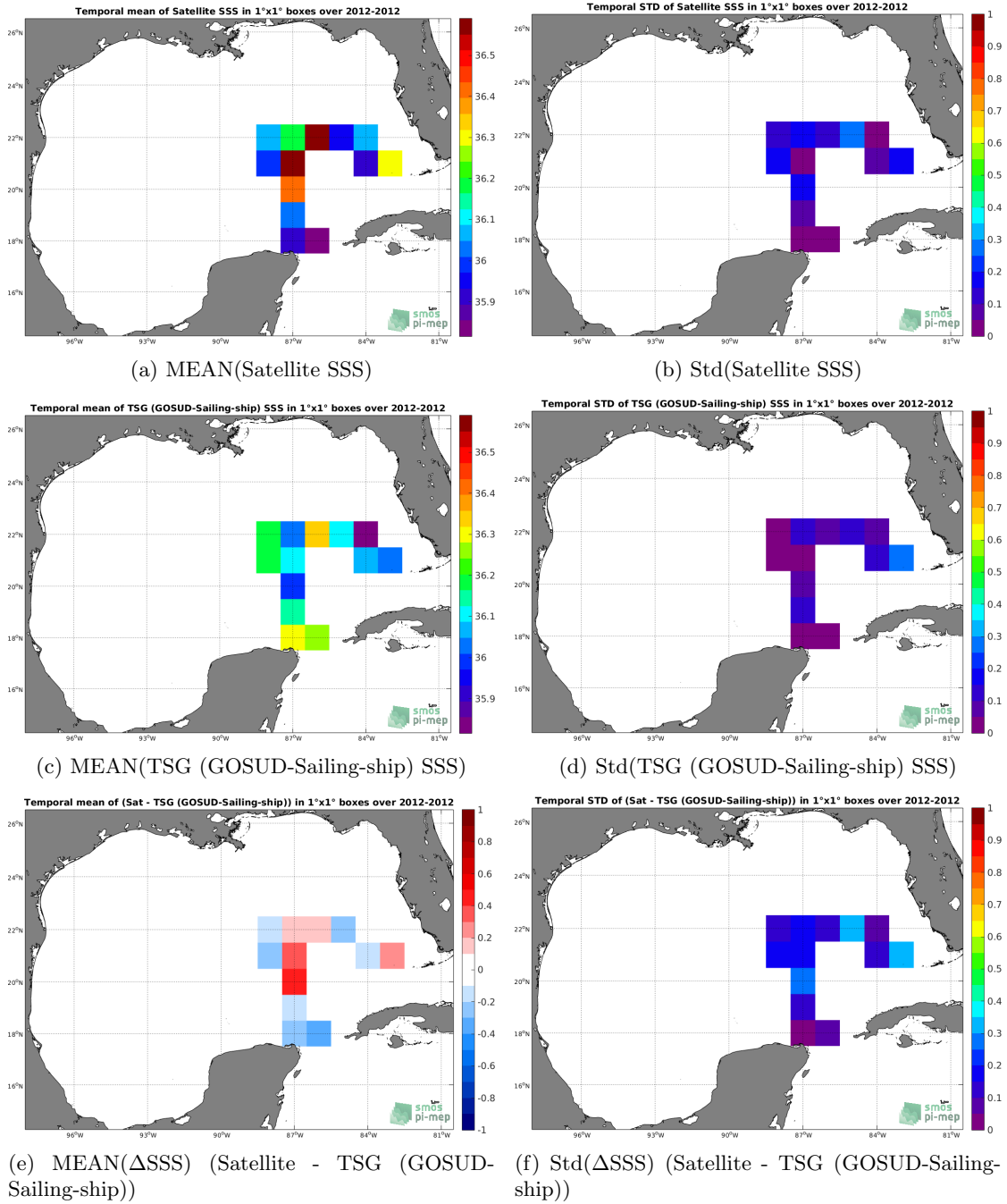
Figure 6: Temporal mean (left) and Std (right) of SSS from SMOS SSS L3 v317 - 10 Days - 25 km (CATDS-CPDC) (top), TSG (GOSUD-Sailing-ship) (middle), and of \Delta SSS (Satellite - TSG (GOSUD-Sailing-ship)). Only match-up pairs are used to generate these maps.
