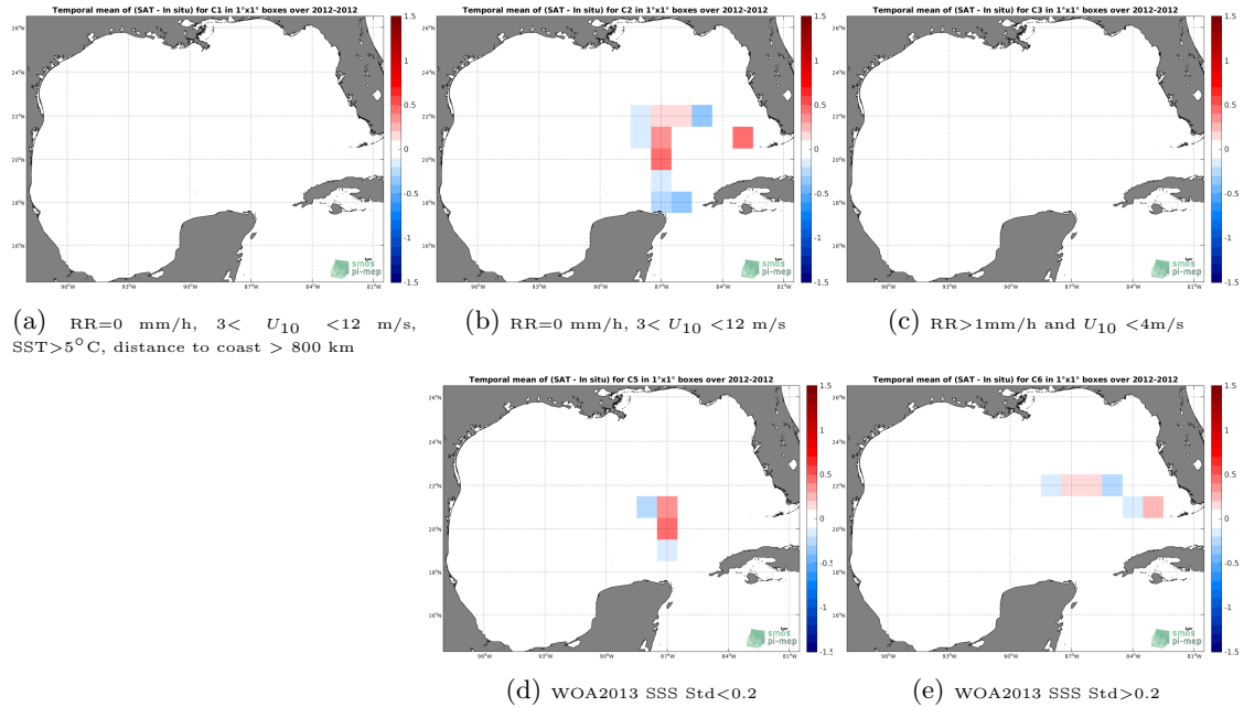
Figure 12: Temporal mean gridded over spatial boxes of size 1^\circ \times 1^\circ of \Delta SSS (SMOS SSS L3 v317 - 10 Days - 25 km (CATDS-CPDC) - TSG (GOSUD-Sailing-ship)) for 5 different subdatasets corresponding to:RR=0 mm/h, 3 < U_{10} < 12 m/s, SST >5^\circ\text{C} , distance to coast > 800 km (a), RR=0 mm/h, 3 < U_{10} < 12 m/s (b), RR >1 mm/h and U_{10} < 4 m/s (c), WOA2013 SSS Std <0.2 (d), WOA2013 SSS Std >0.2 (e).
