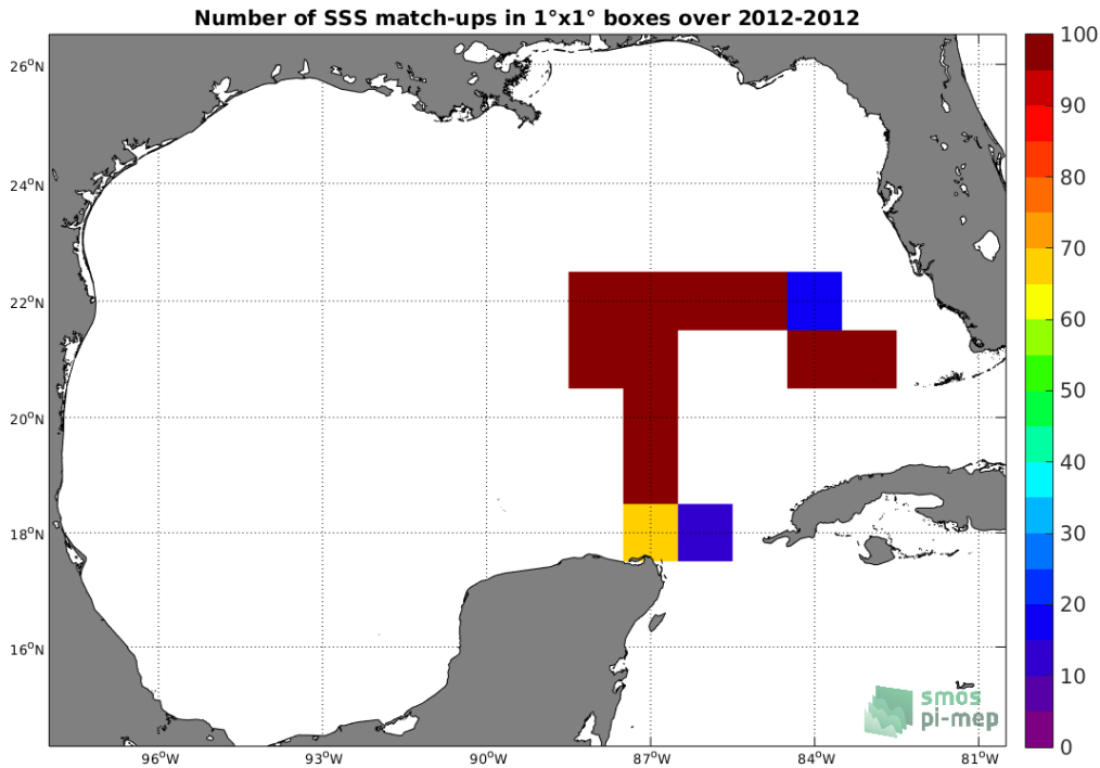
Figure 4: Number of SSS match-ups between TSG (GOSUD-Sailing-ship) SSS and the SMOS SSS L3 v317 - 10 Days - 25 km (CATDS-CPDC) SSS product for the Gulf of Mexico Pi-MEP region over 1^\circ \times 1^\circ boxes and for the full satellite product period.
