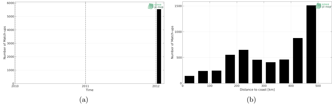
Figure 1: Number of match-ups between TSG (GOSUD-Sailing-ship) and SMOS SSS L3 v317 - 10 Days - 25 km (CATDS-CPDC) SSS as a function of time (a) and as function of the distance to coast (b) over the Gulf of Mexico Pi-MEP region and for the full satellite product period.
