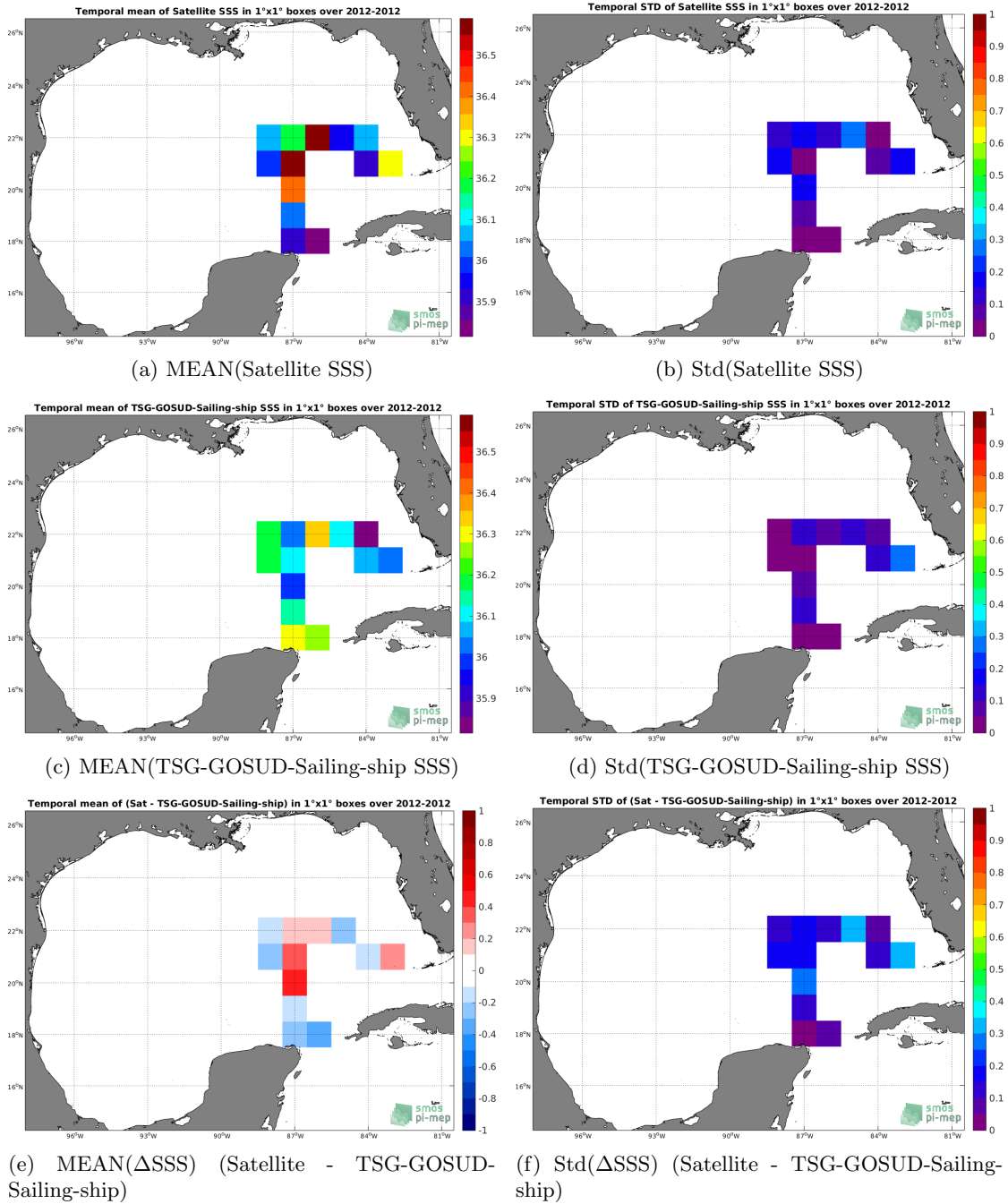
Figure 6: Temporal mean (left) and Std (right) of SSS from SMOS L3 v317 - 10 Days - 25 km (CATDS-CPDC) (top), TSG-GOSUD-Sailing-ship (middle), and of \Delta SSS (Satellite - TSG-GOSUD-Sailing-ship). Only match-up pairs are used to generate these maps.
