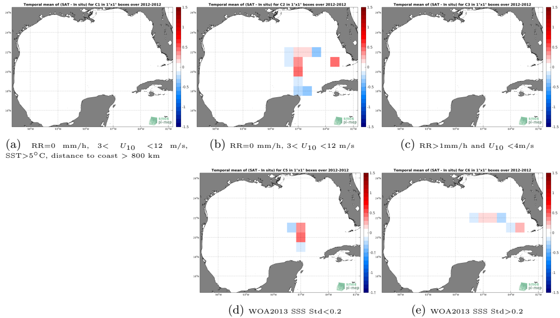
Figure 12: Temporal mean gridded over spatial boxes of size 1^{\circ}\times 1^{\circ} of \Delta SSS (SMOS L3 v317 - 10 Days - 25 km (CATDS-CPDC) - TSG-GOSUD-Sailing-ship) for 5 different subdatasets corresponding to:RR=0 mm/h, 3 < U_{10} < 12 m/s, SST >5^{\circ}\text{C} , distance to coast > 800 km (a), RR=0 mm/h, 3 < U_{10} < 12 m/s (b), RR >1 mm/h and U_{10} < 4 m/s (c), WOA2013 SSS Std <0.2 (d), WOA2013 SSS Std >0.2 (e).
