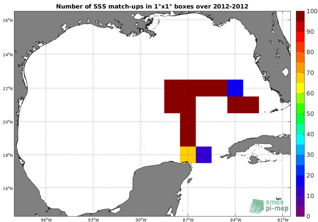
Figure 4: Number of SSS match-ups between TSG-GOSUD-Sailing-ship SSS and the SMOS L3 v317 - 10 Days - 25 km (CATDS-CPDC) SSS product for the Gulf of Mexico Pi-MEP region over 1°x1° boxes and for the full satellite product period.
