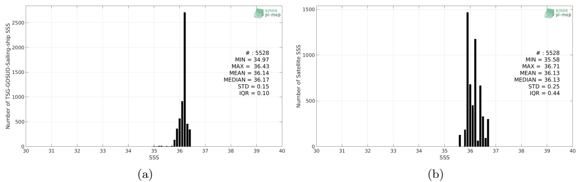
Figure 2: Histograms of SSS from TSG-GOSUD-Sailing-ship (a) and SMOS L3 v317 - 10 Days - 25 km (CATDS-CPDC) (b) considering all match-up pairs per bins of 0.1 over the Gulf of Mexico Pi-MEP region and for the full satellite product period.
