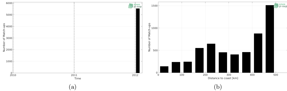
Figure 1: Number of match-ups between TSG-GOSUD-Sailing-ship and SMOS L3 v317 - 10 Days - 25 km (CATDS-CPDC) SSS as a function of time (a) and as function of the distance to coast (b) over the Gulf of Mexico Pi-MEP region and for the full satellite product period.
