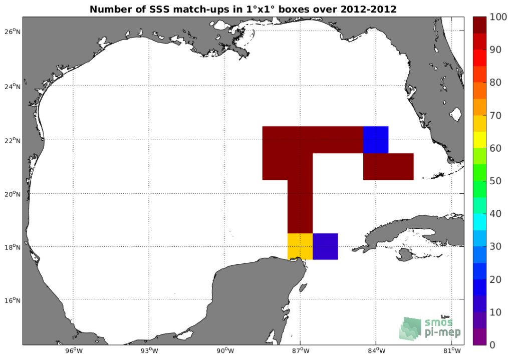
Figure 4: Number of SSS match-ups between TSG-GOSUD-Sailing-ship SSS and the SMOS-L3-CATDS-CPDC-V317-10DAYS-25KM SSS product for the Gulf of Mexico Pi-MEP region over 1°x1° boxes and for the full satellite product period.
