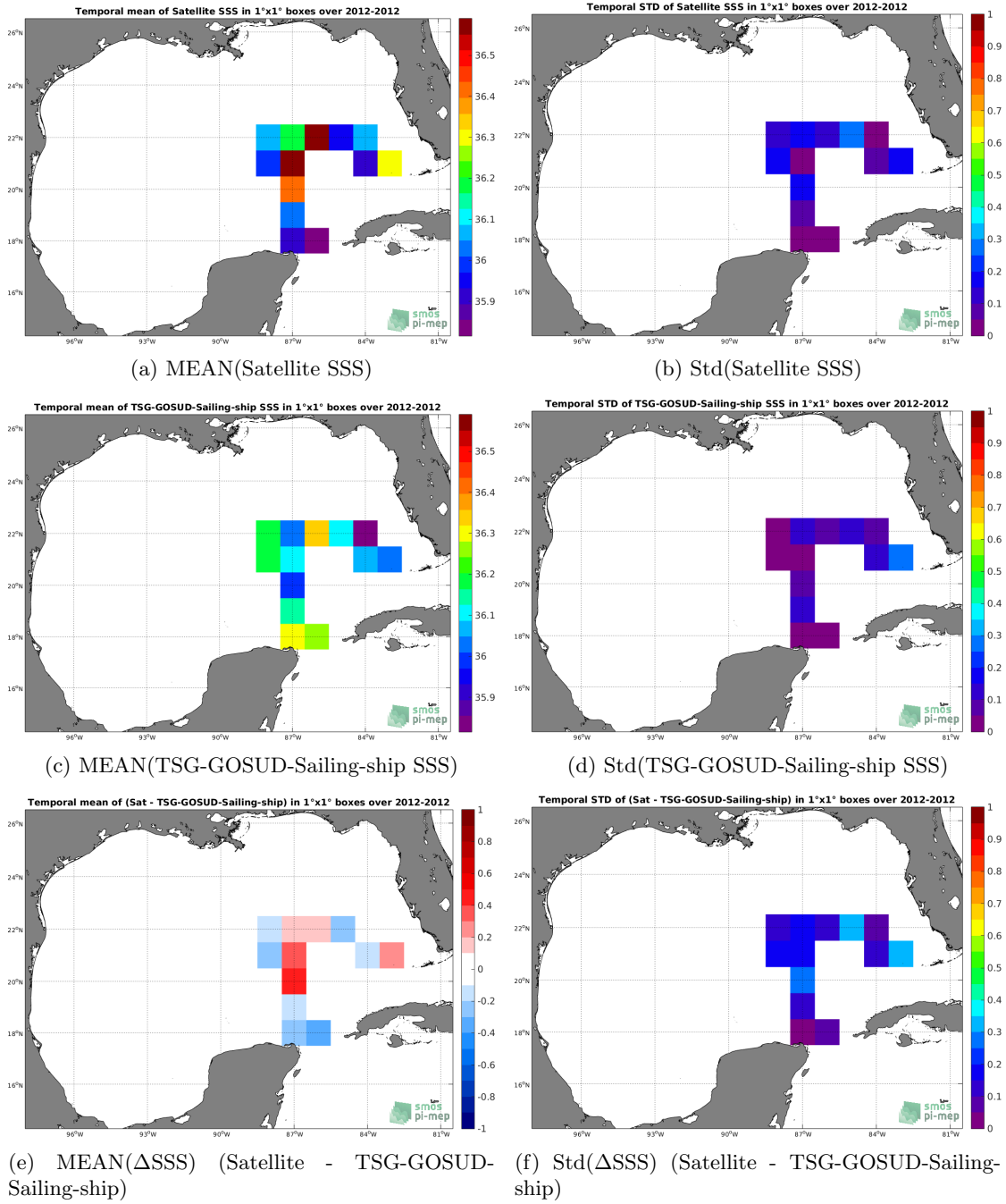
Figure 6: Temporal mean (left) and Std (right) of SSS from SMOS-L3-CATDS-CPDC-V317-10DAYS-25KM (top), TSG-GOSUD-Sailing-ship (middle), and of \Delta SSS (Satellite - TSG-GOSUD-Sailing-ship). Only match-up pairs are used to generate these maps.
