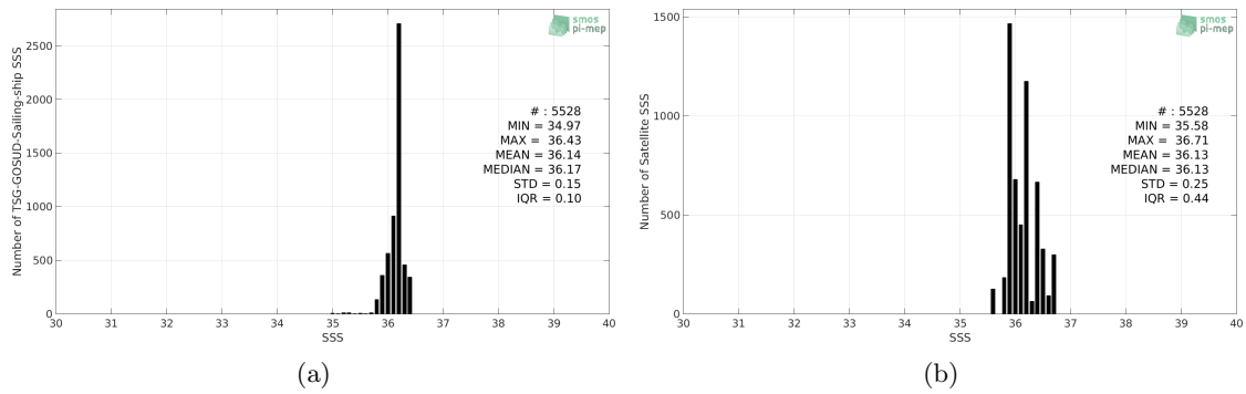
Figure 2: Histograms of SSS from TSG-GOSUD-Sailing-ship (a) and SMOS-L3-CATDS-CPDC-V317-10DAYS-25KM (b) considering all match-up pairs per bins of 0.1 over the Gulf of Mexico Pi-MEP region and for the full satellite product period.
