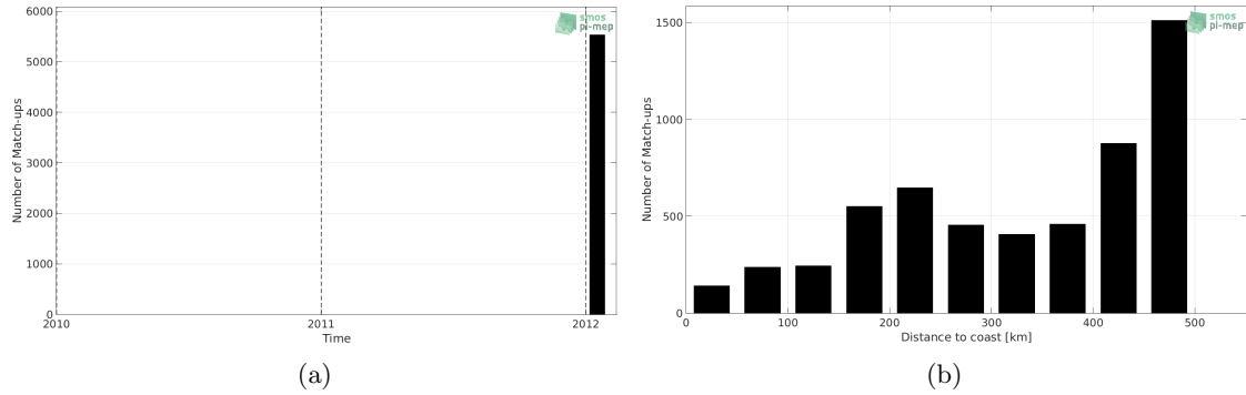
Figure 1: Number of match-ups between TSG-GOSUD-Sailing-ship and SMOS-L3-CATDS-CPDC-V317-10DAYS-25KM SSS as a function of time (a) and as function of the distance to coast (b) over the Gulf of Mexico Pi-MEP region and for the full satellite product period.
