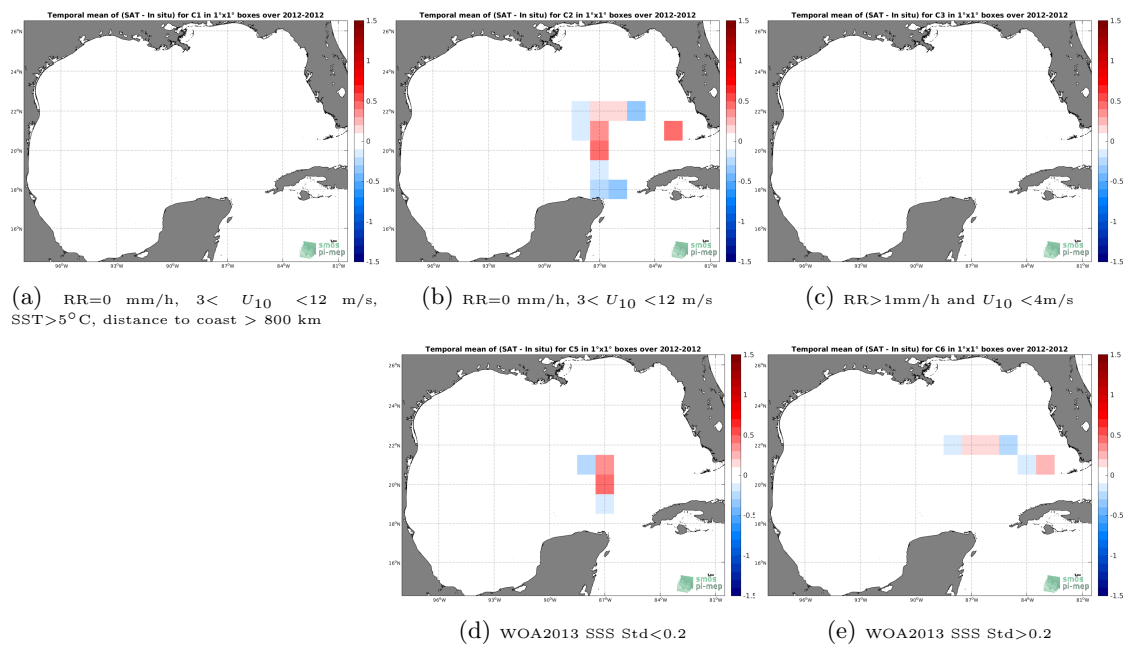
Figure 12: Temporal mean gridded over spatial boxes of size 1^\circ \times 1^\circ of \Delta SSS (SMOS-L3-CATDS-CPDC-V317-10DAYS-25KM - TSG-GOSUD-Sailing-ship) for 5 different subdatasets corresponding to:RR=0 mm/h, 3 < U_{10} < 12 m/s, SST>5°C, distance to coast > 800 km (a), RR=0 mm/h, 3 < U_{10} < 12 m/s (b), RR>1mm/h and U_{10} < 4 m/s (c), WOA2013 SSS Std<0.2 (d), WOA2013 SSS Std>0.2 (e).
