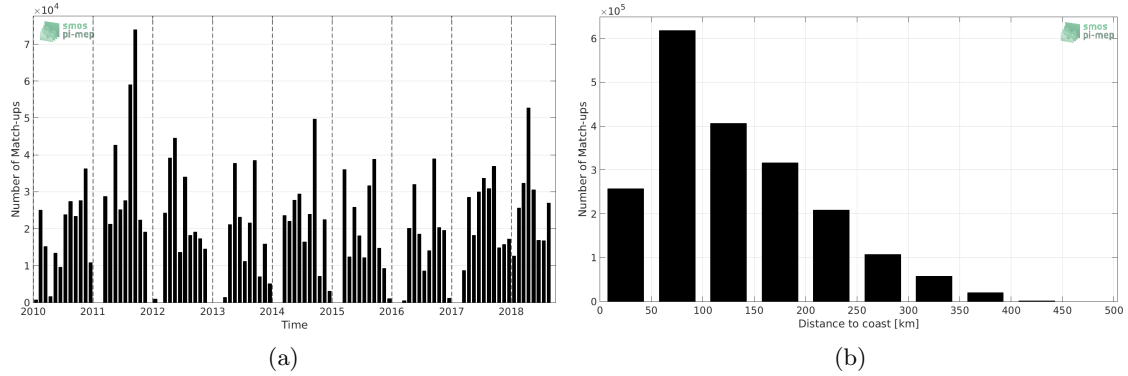
Figure 1: Number of match-ups between TSG-SAMOS and SMOS-L3-CATDS-CPDC-V3-MONTHLY-25KM SSS as a function of time (a) and as function of the distance to coast (b) over the Gulf of Mexico Pi-MEP region and for the full satellite product period.
