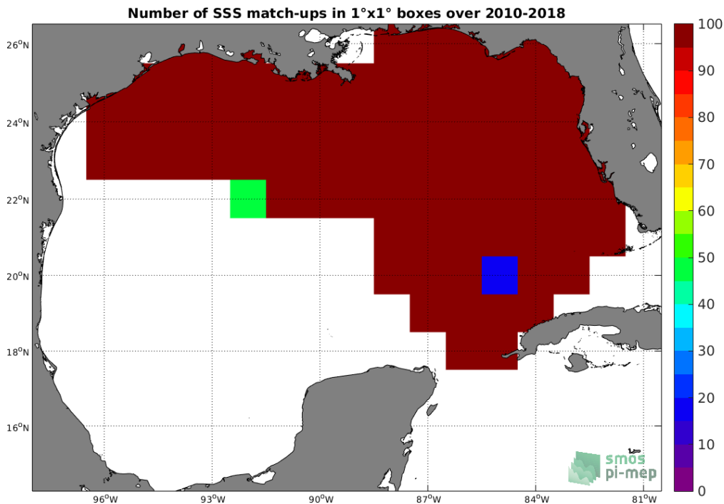
Figure 4: Number of SSS match-ups between TSG-SAMOS SSS and the SMOS-L3-CATDS-CPDC-V3-MONTHLY-25KM SSS product for the Gulf of Mexico Pi-MEP region over 1^\circ \times 1^\circ boxes and for the full satellite product period.
