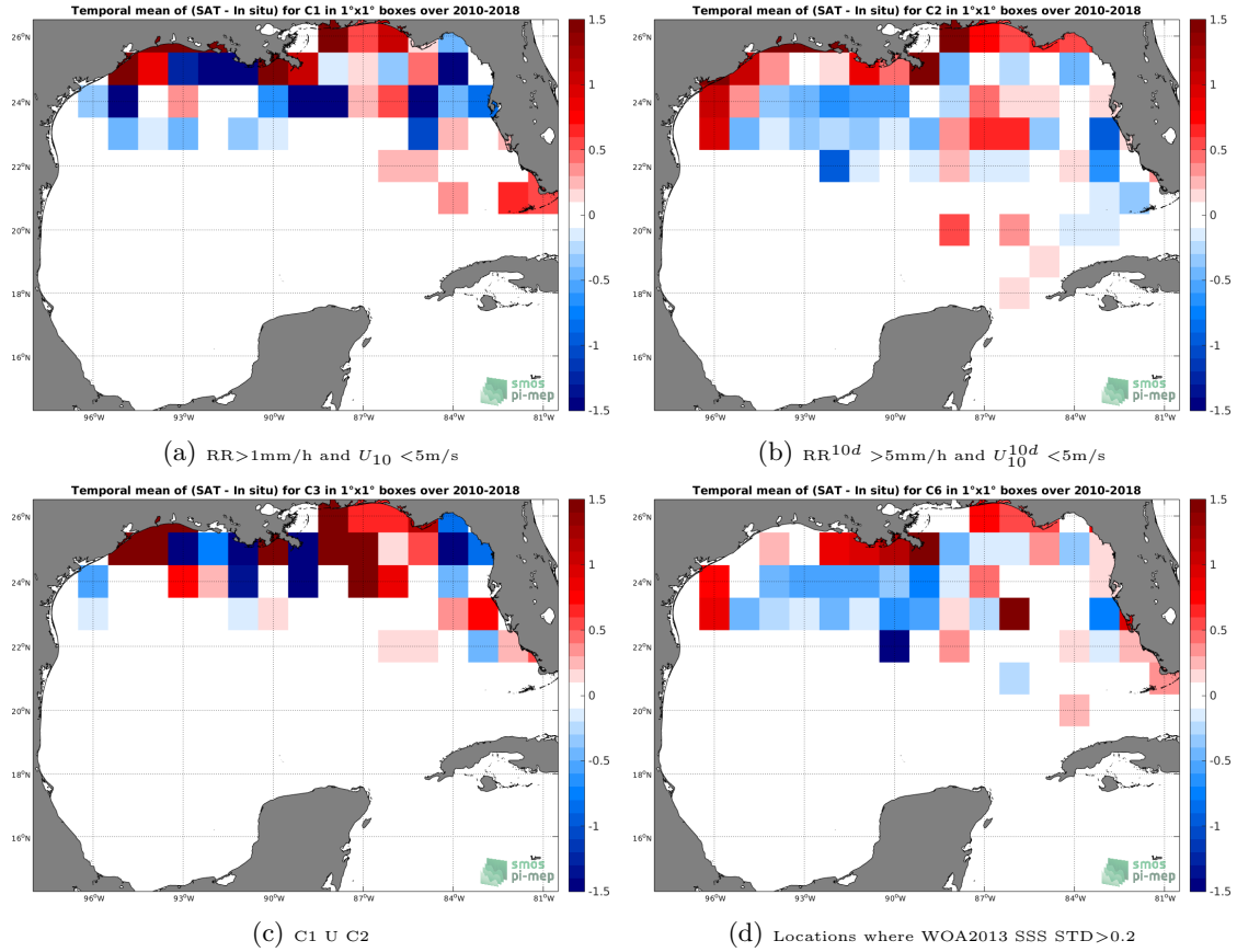
Figure 12: Temporal mean gridded over spatial boxes of size 1^\circ \times 1^\circ of \Delta SSS (SMOS-L3-CATDS-CPDC-V3-MONTHLY-25KM - TSG-SAMOS) for 4 different subdatasets corresponding to: RR > 1\text{mm/h} and U_{10} < 5\text{m/s} (a), RR^{10d} > 5\text{mm/h} and U_{10}^{10d} < 5\text{m/s} (b), C1 U C2 (c), Locations where WOA2013 SSS STD > 0.2 (d).
