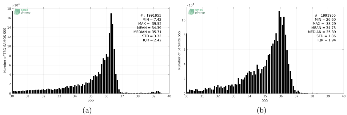
Figure 2: Histograms of SSS from TSG-SAMOS (a) and SMOS-L3-CATDS-CPDC-V3-MONTHLY-25KM (b) considering all match-up pairs per bins of 0.1 over the Gulf of Mexico Pi-MEP region and for the full satellite product period.
