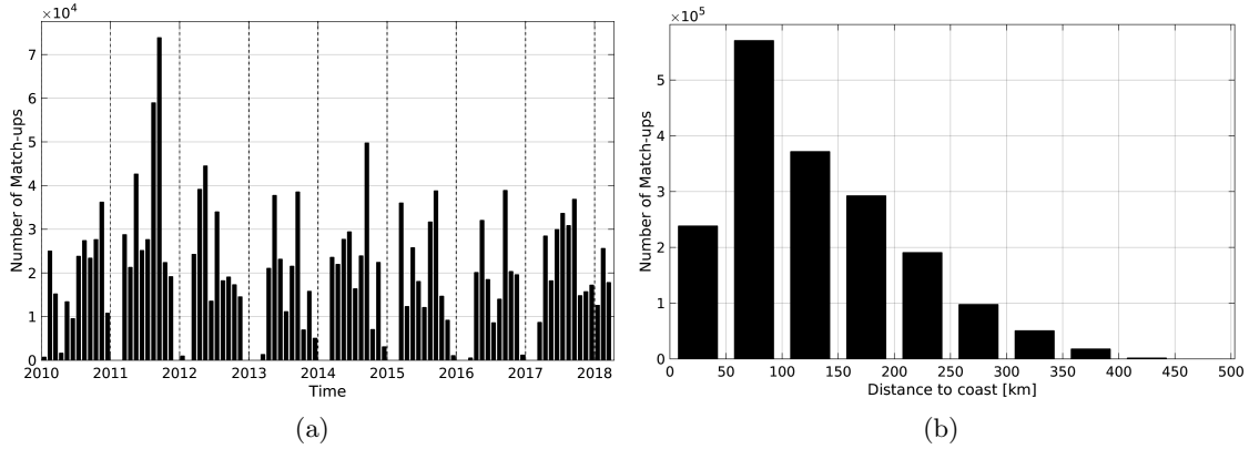
Figure 1: Number of match-ups between TSG-SAMOS and SMOS-L3-CATDS-CPDC-V3-MONTHLY-25KM SSS as a function of time (a) and as function of the distance to coast (b) over the Gulf of Mexico Pi-MEP region and for the full satellite product period.
