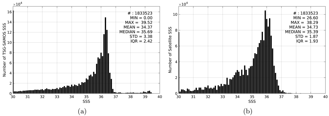
Figure 2: Histograms of SSS from TSG-SAMOS (a) and SMOS-L3-CATDS-CPDC-V3-MONTHLY-25KM (b) considering all match-up pairs per bins of 0.1 over the Gulf of Mexico Pi-MEP region and for the full satellite product period.
