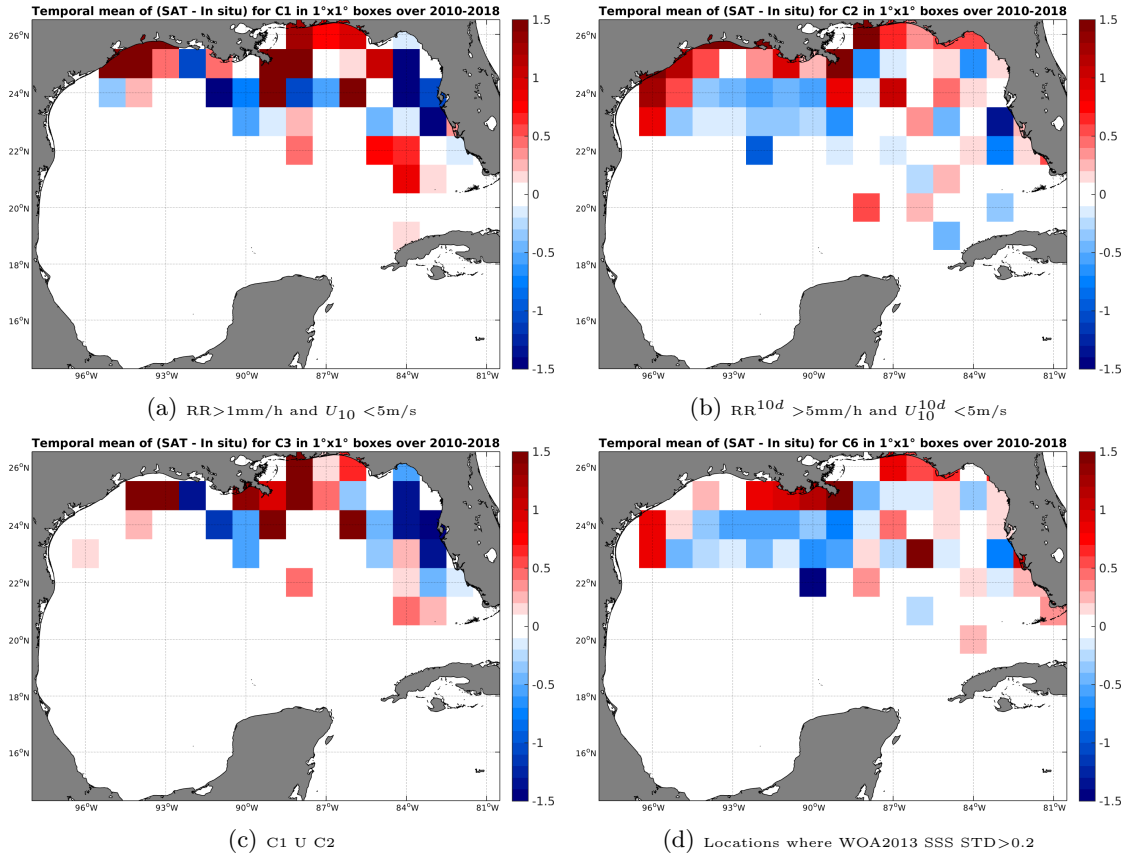
Figure 12: Temporal mean gridded over spatial boxes of size 1^\circ \times 1^\circ of \Delta SSS (SMOS-L3-CATDS-CPDC-V3-MONTHLY-25KM - TSG-SAMOS) for 4 different subdatasets corresponding to: RR > 1mm/h and U_{10} < 5\text{m/s} (a), RR^{10d} > 5\text{mm/h} and U_{10}^{10d} < 5\text{m/s} (b), C1 U C2 (c), Locations where WOA2013 SSS STD > 0.2 (d).
