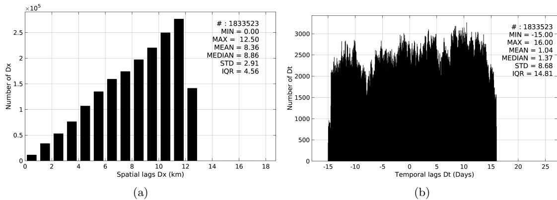
Figure 5: Histograms of the spatial (a) and temporal (b) lags between the time of the TSG-SAMOS measurements and the date of the corresponding SMOS-L3-CATDS-CPDC-V3-MONTHLY-25KM SSS product.
