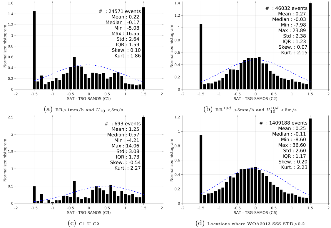
Figure 13: Normalized histogram of \Delta SSS (SMOS-L3-CATDS-CPDC-V3-MONTHLY-25KM - TSG-SAMOS) for 6 different subdatasets corresponding to: RR > 1mm/h and U_{10} < 5 m/s (a), RR^{10d} > 5 mm/h and U_{10}^{10d} < 5 m/s (b), C1 U C2 (c), Locations where WOA2013 SSS STD > 0.2 (d).
