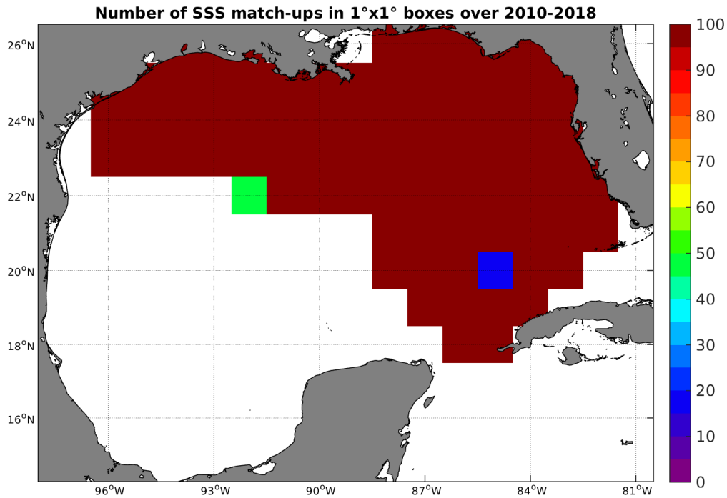
Figure 4: Number of SSS match-ups between TSG-SAMOS SSS and the SMOS-L3-CATDS-CPDC-V3-MONTHLY-25KM SSS product for the Gulf of Mexico Pi-MEP region over 1^\circ \times 1^\circ boxes and for the full satellite product period.
