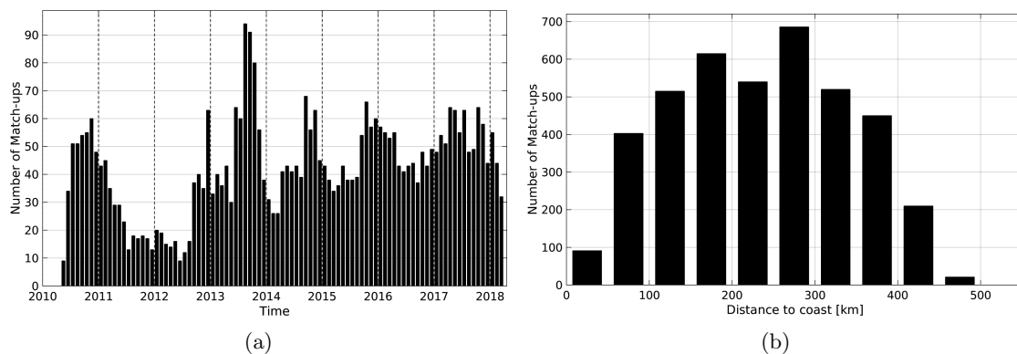
Figure 1: Number of match-ups between Argo and SMOS-L3-CATDS-CPDC-V3-MONTHLY-25KM SSS as a function of time (a) and as function of the distance to coast (b) over the Gulf of Mexico Pi-MEP region and for the full satellite product period.
