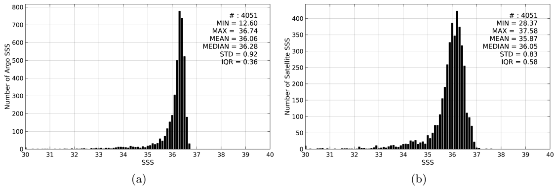
Figure 2: Histograms of SSS from Argo (a) and SMOS-L3-CATDS-CPDC-V3-MONTHLY-25KM (b) considering all match-up pairs per bins of 0.1 over the Gulf of Mexico Pi-MEP region and for the full satellite product period.
