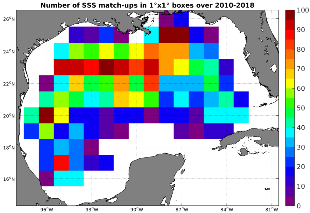
Figure 4: Number of SSS match-ups between Argo SSS and the SMOS-L3-CATDS-CPDC-V3-MONTHLY-25KM SSS product for the Gulf of Mexico Pi-MEP region over 1^\circ \times 1^\circ boxes and for the full satellite product period.
