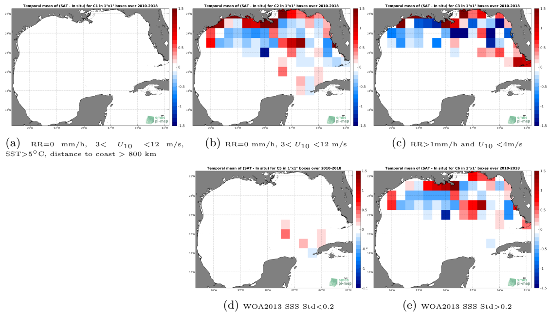
Figure 12: Temporal mean gridded over spatial boxes of size 1^\circ \times 1^\circ of \Delta SSS (SMOS-L3-CATDS-CPDC-V3-10DAYS-25KM - TSG-SAMOS) for 5 different subdatasets corresponding to:RR=0 mm/h, 3 < U_{10} < 12 m/s, SST >5^\circ C, distance to coast > 800 km (a), RR=0 mm/h, 3 < U_{10} < 12 m/s (b), RR >1 mm/h and U_{10} < 4 m/s (c), WOA2013 SSS Std <0.2 (d), WOA2013 SSS Std >0.2 (e).
