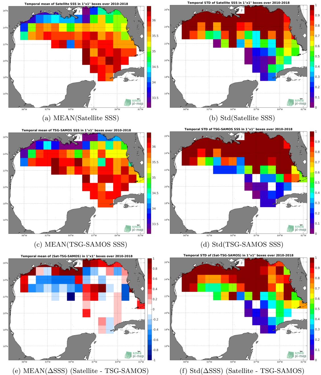
Figure 6: Temporal mean (left) and Std (right) of SSS from SMOS-L3-CATDS-CPDC-V3-10DAYS-25KM (top), TSG-SAMOS (middle), and of \Delta SSS (Satellite - TSG-SAMOS). Only match-up pairs are used to generate these maps.
