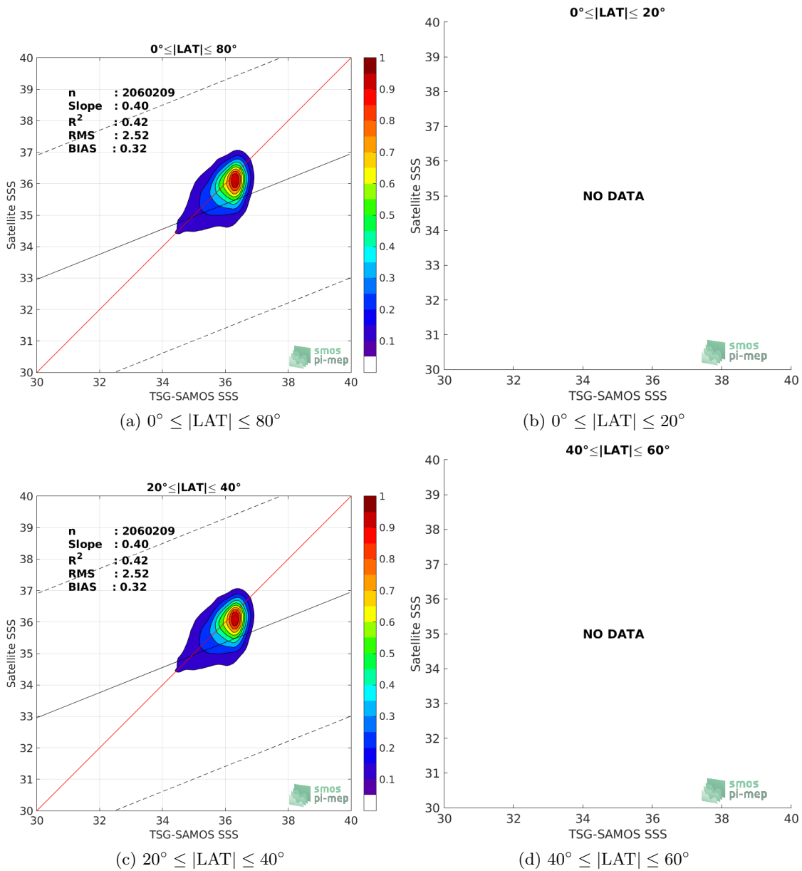
Figure 9: Contour maps of the concentration of SMOS-L3-CATDS-CPDC-V3-10DAYS-25KM SSS (y-axis) versus TSG-SAMOS SSS (x-axis) at match-up pairs for different latitude bands. For each plot, the red line shows x=y . The black thin and dashed lines indicate a linear fit through the data cloud and the \pm 95\% confidence levels, respectively. The number match-up pairs n , the slope and R^2 coefficient of the linear fit, the root mean square (RMS) and the mean bias between satellite and in situ data are indicated for each latitude band in each plots.
