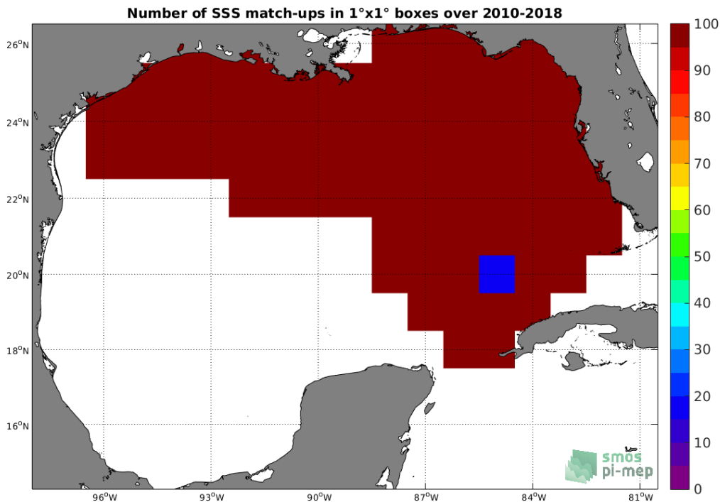
Figure 4: Number of SSS match-ups between TSG-SAMOS SSS and the SMOS-L3-CATDS-CPDC-V3-10DAYS-25KM SSS product for the Gulf of Mexico Pi-MEP region over 1^\circ \times 1^\circ boxes and for the full satellite product period.
