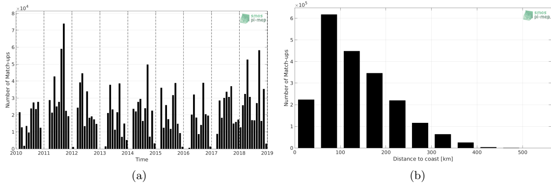
Figure 1: Number of match-ups between TSG-SAMOS and SMOS-L3-CATDS-CPDC-V3-10DAYS-25KM SSS as a function of time (a) and as function of the distance to coast (b) over the Gulf of Mexico Pi-MEP region and for the full satellite product period.
