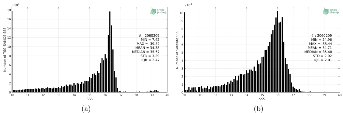
Figure 2: Histograms of SSS from TSG-SAMOS (a) and SMOS-L3-CATDS-CPDC-V3-10DAYS-25KM (b) considering all match-up pairs per bins of 0.1 over the Gulf of Mexico Pi-MEP region and for the full satellite product period.
