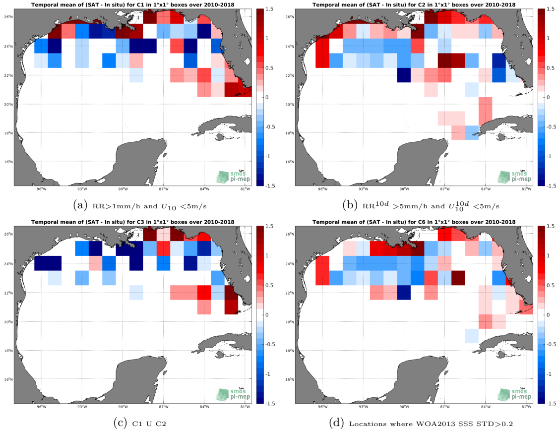
Figure 12: Temporal mean gridded over spatial boxes of size 1^\circ \times 1^\circ of \Delta SSS (SMOS-L3-CATDS-CPDC-V3-10DAYS-25KM - TSG-SAMOS) for 4 different subdatasets corresponding to: RR > 1\text{mm/h} and U_{10} < 5\text{m/s} (a), RR^{10d} > 5\text{mm/h} and U_{10}^{10d} < 5\text{m/s} (b), C1 U C2 (c), Locations where WOA2013 SSS STD > 0.2 (d).
