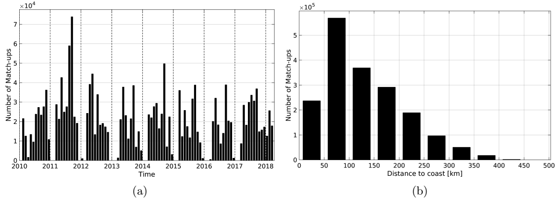
Figure 1: Number of match-ups between TSG-SAMOS and SMOS-L3-CATDS-CPDC-V3-10DAYS-25KM SSS as a function of time (a) and as function of the distance to coast (b) over the Gulf of Mexico Pi-MEP region and for the full satellite product period.
