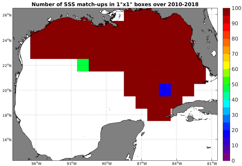
Figure 4: Number of SSS match-ups between TSG-SAMOS SSS and the SMOS-L3-CATDS-CPDC-V3-10DAYS-25KM SSS product for the Gulf of Mexico Pi-MEP region over 1^\circ \times 1^\circ boxes and for the full satellite product period.
