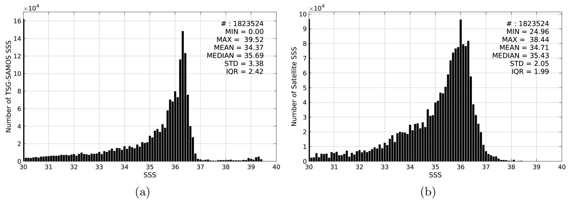
Figure 2: Histograms of SSS from TSG-SAMOS (a) and SMOS-L3-CATDS-CPDC-V3-10DAYS-25KM (b) considering all match-up pairs per bins of 0.1 over the Gulf of Mexico Pi-MEP region and for the full satellite product period.
