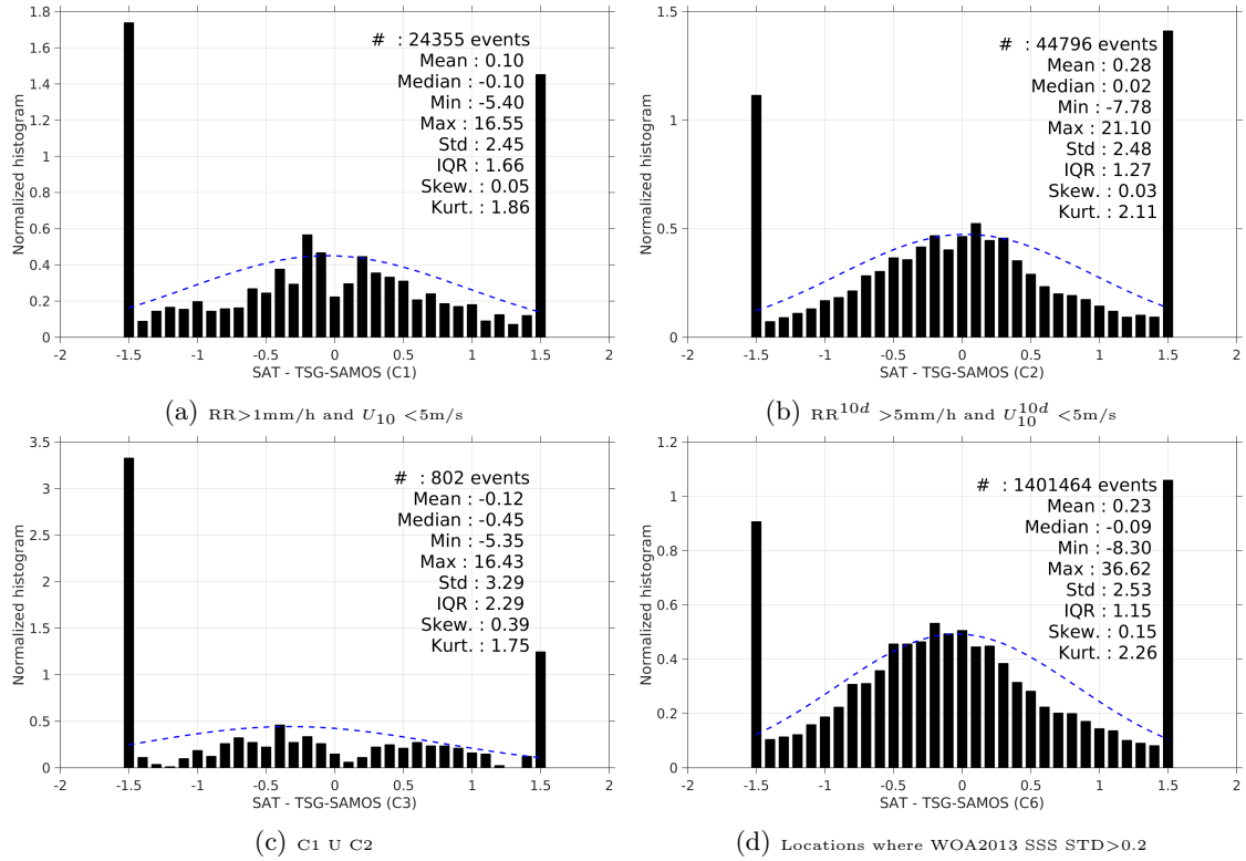
Figure 13: Normalized histogram of \Delta SSS (SMOS-L3-CATDS-CPDC-V3-10DAYS-25KM - TSG-SAMOS) for 6 different subdatasets corresponding to: RR > 1mm/h and U_{10} < 5 m/s (a), RR^{10d} > 5 mm/h and U_{10}^{10d} < 5 m/s (b), C1 U C2 (c), Locations where WOA2013 SSS STD > 0.2 (d).
