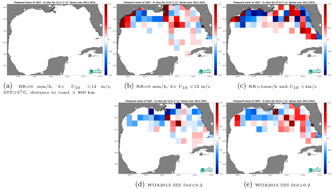
Figure 12: Temporal mean gridded over spatial boxes of size 1^{\circ}\times 1^{\circ} of \Delta\text{SSS} (SMOS SSS L3 v2 - 9-Days (BEC) - TSG (SAMOS)) for 5 different subdatasets corresponding to:RR=0 mm/h, 3 < U_{10} < 12 m/s, SST >5^{\circ}\text{C} , distance to coast > 800 km (a), RR=0 mm/h, 3 < U_{10} < 12 m/s (b), RR >1 mm/h and U_{10} < 4 m/s (c), WOA2013 SSS Std <0.2 (d), WOA2013 SSS Std >0.2 (e).
