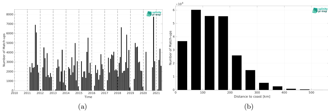
Figure 1: Number of match-ups between TSG (SAMOS) and SMOS SSS L3 v2 - 9-Days (BEC) SSS as a function of time (a) and as function of the distance to coast (b) over the Gulf of Mexico Pi-MEP region and for the full satellite product period.
