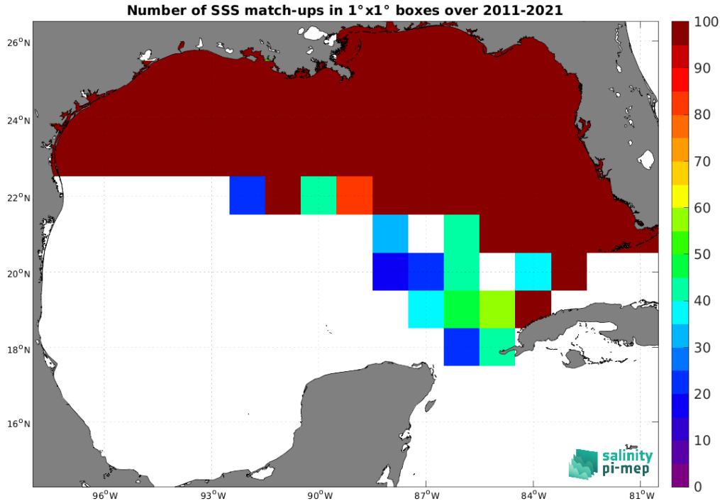
Figure 4: Number of SSS match-ups between TSG (SAMOS) SSS and the SMOS SSS L3 v2 - 9-Days (BEC) SSS product for the Gulf of Mexico Pi-MEP region over 1^\circ \times 1^\circ boxes and for the full satellite product period.
