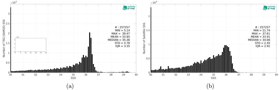
Figure 2: Histograms of SSS from TSG (SAMOS) (a) and SMOS SSS L3 v2 - 9-Days (BEC) (b) considering all match-up pairs per bins of 0.1 over the Gulf of Mexico Pi-MEP region and for the full satellite product period.
