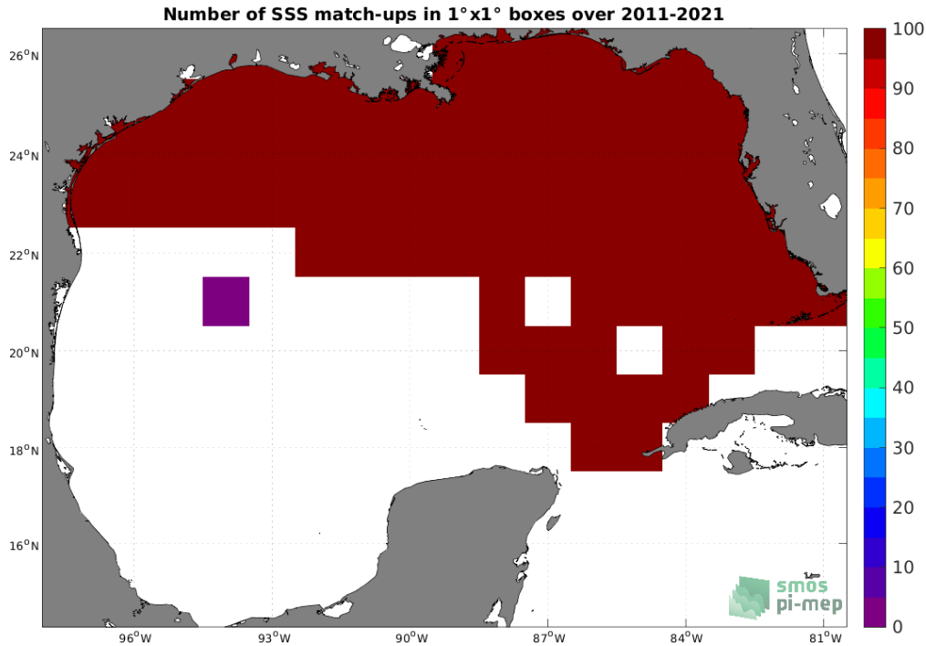
Figure 4: Number of SSS match-ups between TSG (SAMOS) SSS and the SMOS SSS L3 v2 - 9-Days (BEC) SSS product for the Gulf of Mexico Pi-MEP region over 1^{\circ} \times 1^{\circ} boxes and for the full satellite product period.
