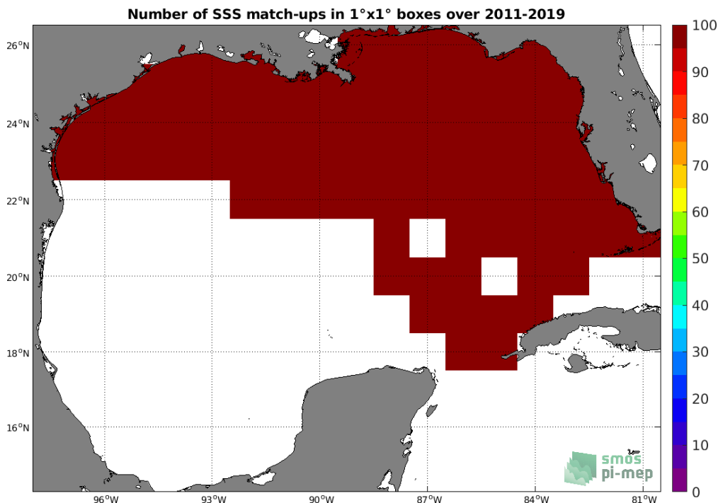
Figure 4: Number of SSS match-ups between TSG (SAMOS) SSS and the SMOS SSS L3 v2 - 9-Days (BEC) SSS product for the Gulf of Mexico Pi-MEP region over 1°x1° boxes and for the full satellite product period.
