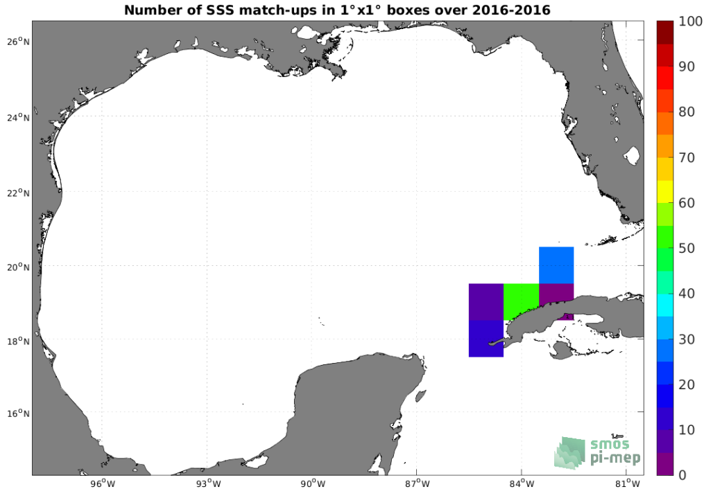
Figure 4: Number of SSS match-ups between TSG (LEGOS-DM) SSS and the SMOS SSS L3 v2 - 9-Days (BEC) SSS product for the Gulf of Mexico Pi-MEP region over 1^\circ \times 1^\circ boxes and for the full satellite product period.
