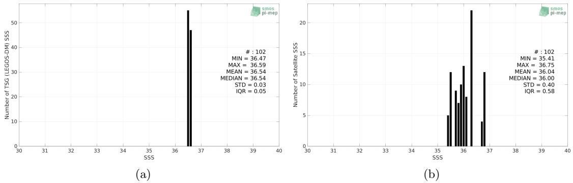
Figure 2: Histograms of SSS from TSG (LEGOS-DM) (a) and SMOS SSS L3 v2 - 9-Days (BEC) (b) considering all match-up pairs per bins of 0.1 over the Gulf of Mexico Pi-MEP region and for the full satellite product period.
