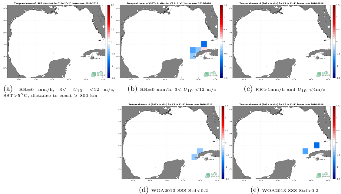
Figure 12: Temporal mean gridded over spatial boxes of size 1^{\circ}\times 1^{\circ} of \Delta\text{SSS} (SMOS SSS L3 v2 - 9-Days (BEC) - TSG (LEGOS-DM)) for 5 different subdatasets corresponding to:RR=0 mm/h, 3 < U_{10} < 12 m/s, SST >5^{\circ}\text{C} , distance to coast > 800 km (a), RR=0 mm/h, 3 < U_{10} < 12 m/s (b), RR >1 mm/h and U_{10} < 4 m/s (c), WOA2013 SSS Std <0.2 (d), WOA2013 SSS Std >0.2 (e).
