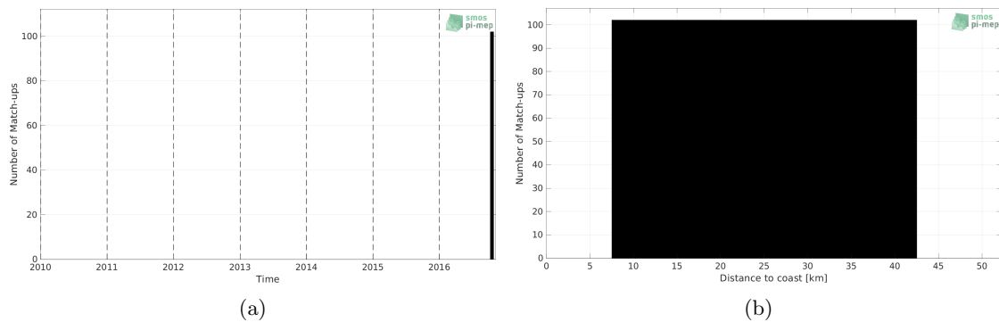
Figure 1: Number of match-ups between TSG (LEGOS-DM) and SMOS SSS L3 v2 - 9-Days (BEC) SSS as a function of time (a) and as function of the distance to coast (b) over the Gulf of Mexico Pi-MEP region and for the full satellite product period.
