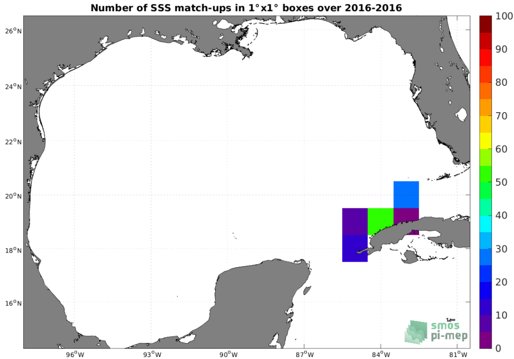
Figure 4: Number of SSS match-ups between TSG (LEGOS-DM) SSS and the SMOS SSS L3 v2 - 9-Days (BEC) SSS product for the Gulf of Mexico Pi-MEP region over 1°×1° boxes and for the full satellite product period.
