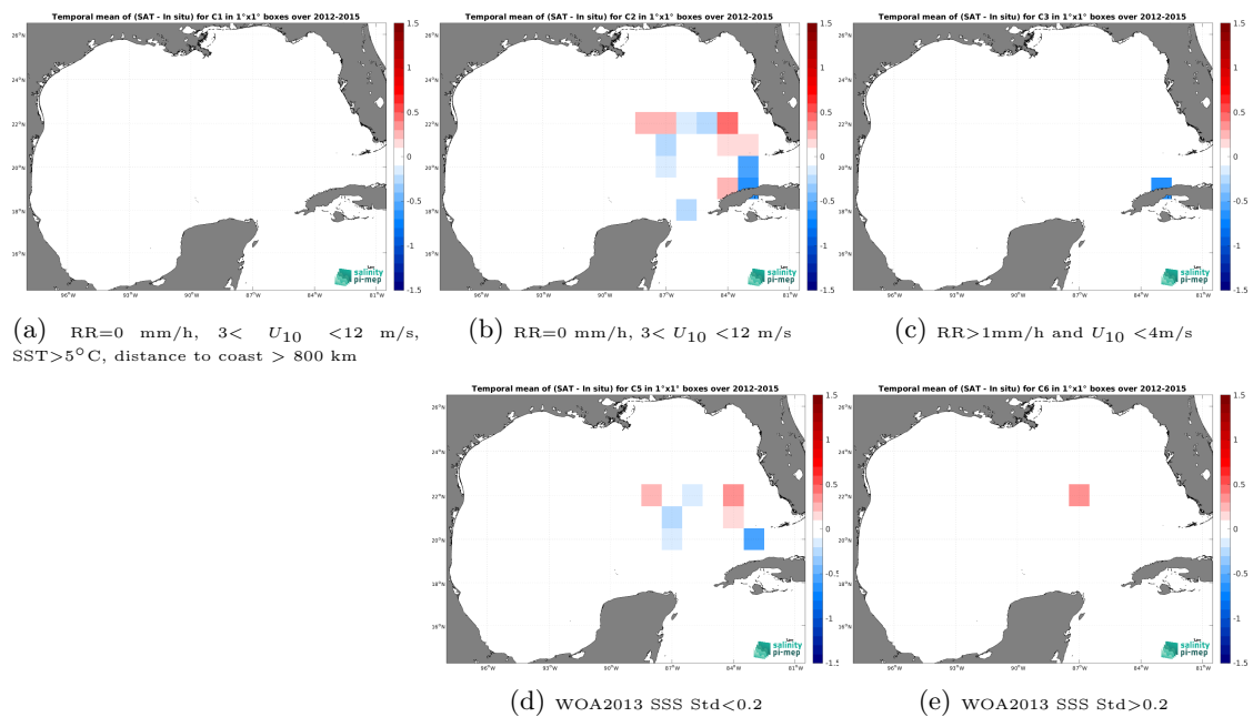
Figure 14: Temporal mean gridded over spatial boxes of size 1^\circ \times 1^\circ of \Delta SSS (SMOS SSS L3 v2 - 9-Days (BEC) - TSG (GOSUD-Sailing-ship)) for 5 different subdatasets corresponding to:RR=0 mm/h, 3 < U_{10} < 12 m/s, SST > 5^\circ\text{C} , distance to coast > 800 km (a), RR=0 mm/h, 3 < U_{10} < 12 m/s (b), RR > 1 mm/h and U_{10} < 4 m/s (c), WOA2013 SSS Std < 0.2 (d), WOA2013 SSS Std > 0.2 (e).
