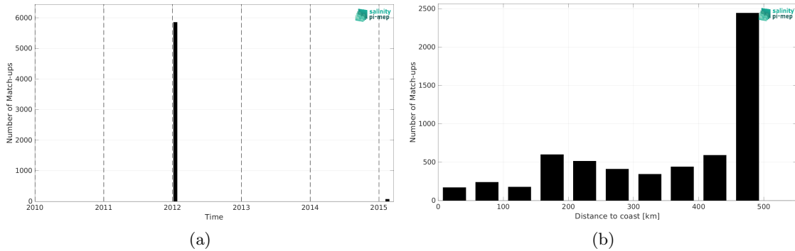
Figure 2: Number of match-ups between TSG (GOSUD-Sailing-ship) and SMOS SSS L3 v2 - 9-Days (BEC) SSS as a function of time (a) and as function of the distance to coast (b) over the Gulf of Mexico Pi-MEP region and for the full satellite product period.
