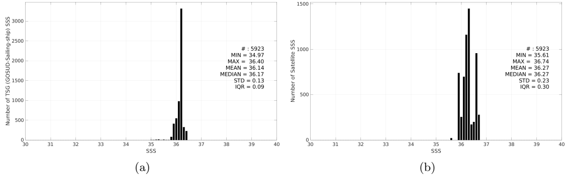
Figure 3: Histograms of SSS from TSG (GOSUD-Sailing-ship) (a) and SMOS SSS L3 v2 - 9-Days (BEC) (b) considering all match-up pairs per bins of 0.1 over the Gulf of Mexico Pi-MEP region and for the full satellite product period.
