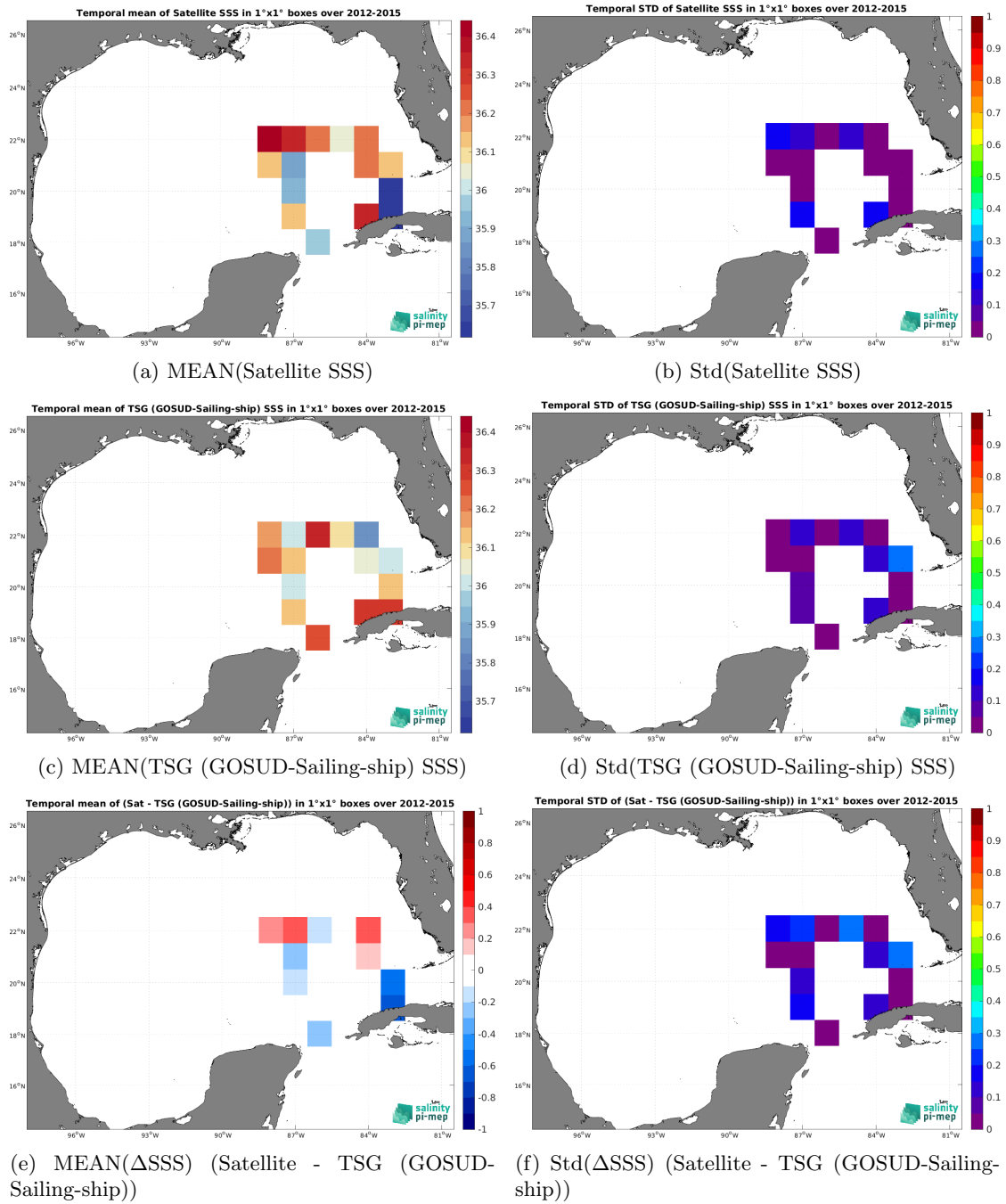
Figure 7: Temporal mean (left) and Std (right) of SSS from SMOS SSS L3 v2 - 9-Days (BEC) (top), TSG (GOSUD-Sailing-ship) (middle), and of \Delta SSS (Satellite - TSG (GOSUD-Sailing-ship)). Only match-up pairs are used to generate these maps.
