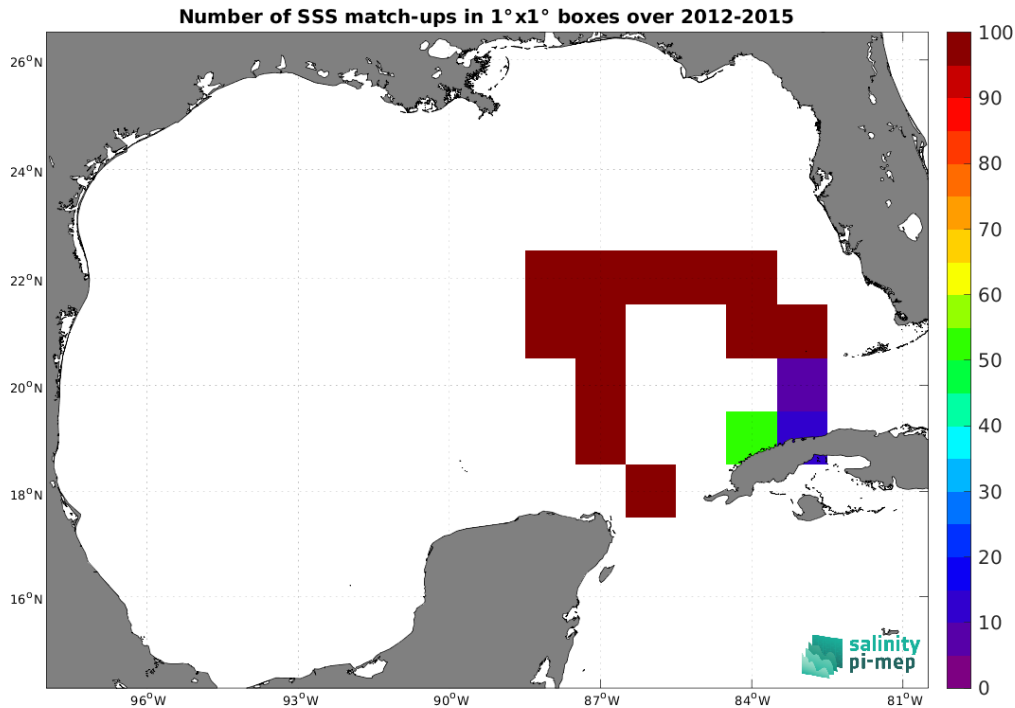
Figure 5: Number of SSS match-ups between TSG (GOSUD-Sailing-ship) SSS and the SMOS SSS L3 v2 - 9-Days (BEC) SSS product for the Gulf of Mexico Pi-MEP region over 1^\circ \times 1^\circ boxes and for the full satellite product period.
