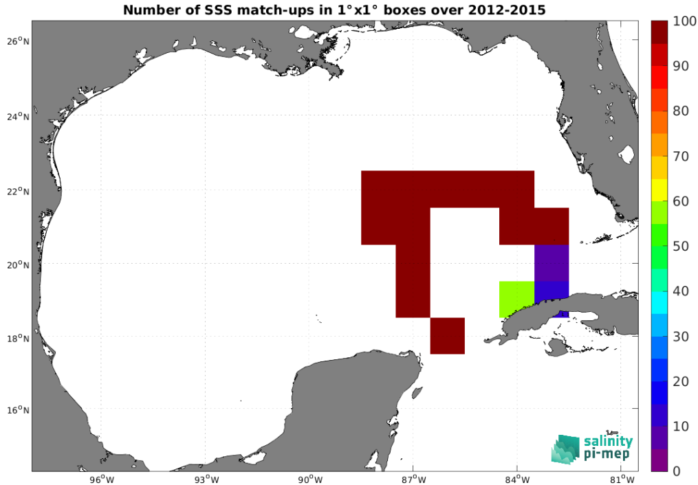
Figure 4: Number of SSS match-ups between TSG (GOSUD-Sailing-ship) SSS and the SMOS SSS L3 v2 - 9-Days (BEC) SSS product for the Gulf of Mexico Pi-MEP region over 1^\circ \times 1^\circ boxes and for the full satellite product period.
