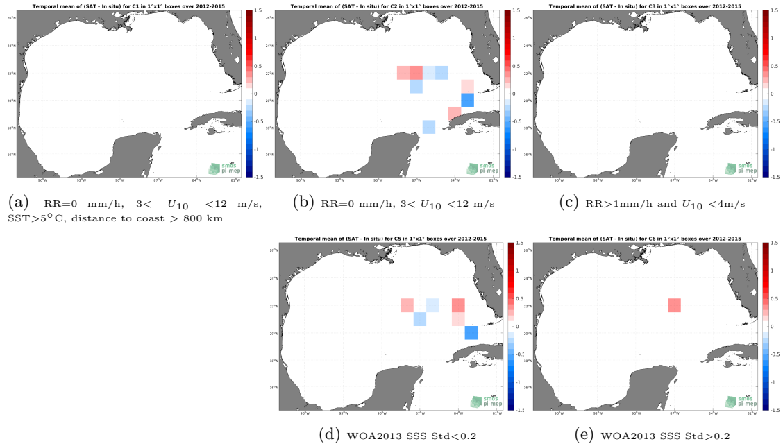
Figure 12: Temporal mean gridded over spatial boxes of size 1^{\circ}\times 1^{\circ} of \Delta SSS (SMOS SSS L3 v2 - 9-Days (BEC) - TSG (GOSUD-Sailing-ship)) for 5 different subdatasets corresponding to:RR=0 mm/h, 3 < U_{10} < 12 m/s, SST >5^{\circ}\text{C} , distance to coast > 800 km (a), RR=0 mm/h, 3 < U_{10} < 12 m/s (b), RR >1 mm/h and U_{10} < 4 m/s (c), WOA2013 SSS Std <0.2 (d), WOA2013 SSS Std >0.2 (e).
