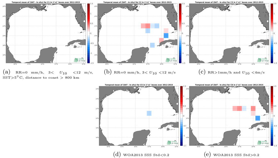
Figure 12: Temporal mean gridded over spatial boxes of size 1^\circ \times 1^\circ of \Delta SSS (SMOS SSS L3 v2 - 9-Days (BEC) - TSG (GOSUD-Sailing-ship)) for 5 different subdatasets corresponding to: RR=0 mm/h, 3 < U_{10} < 12 m/s, SST > 5^\circ\text{C} , distance to coast > 800 km (a), RR=0 mm/h, 3 < U_{10} < 12 m/s (b), RR > 1 mm/h and U_{10} < 4 m/s (c), WOA2013 SSS Std < 0.2 (d), WOA2013 SSS Std > 0.2 (e).
