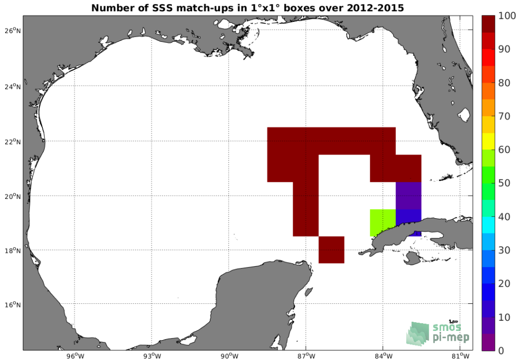
Figure 4: Number of SSS match-ups between TSG (GOSUD-Sailing-ship) SSS and the SMOS SSS L3 v2 - 9-Days (BEC) SSS product for the Gulf of Mexico Pi-MEP region over 1°x1° boxes and for the full satellite product period.
