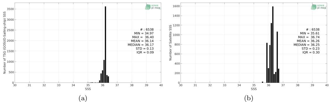
Figure 2: Histograms of SSS from TSG (GOSUD-Sailing-ship) (a) and SMOS SSS L3 v2 - 9-Days (BEC) (b) considering all match-up pairs per bins of 0.1 over the Gulf of Mexico Pi-MEP region and for the full satellite product period.
