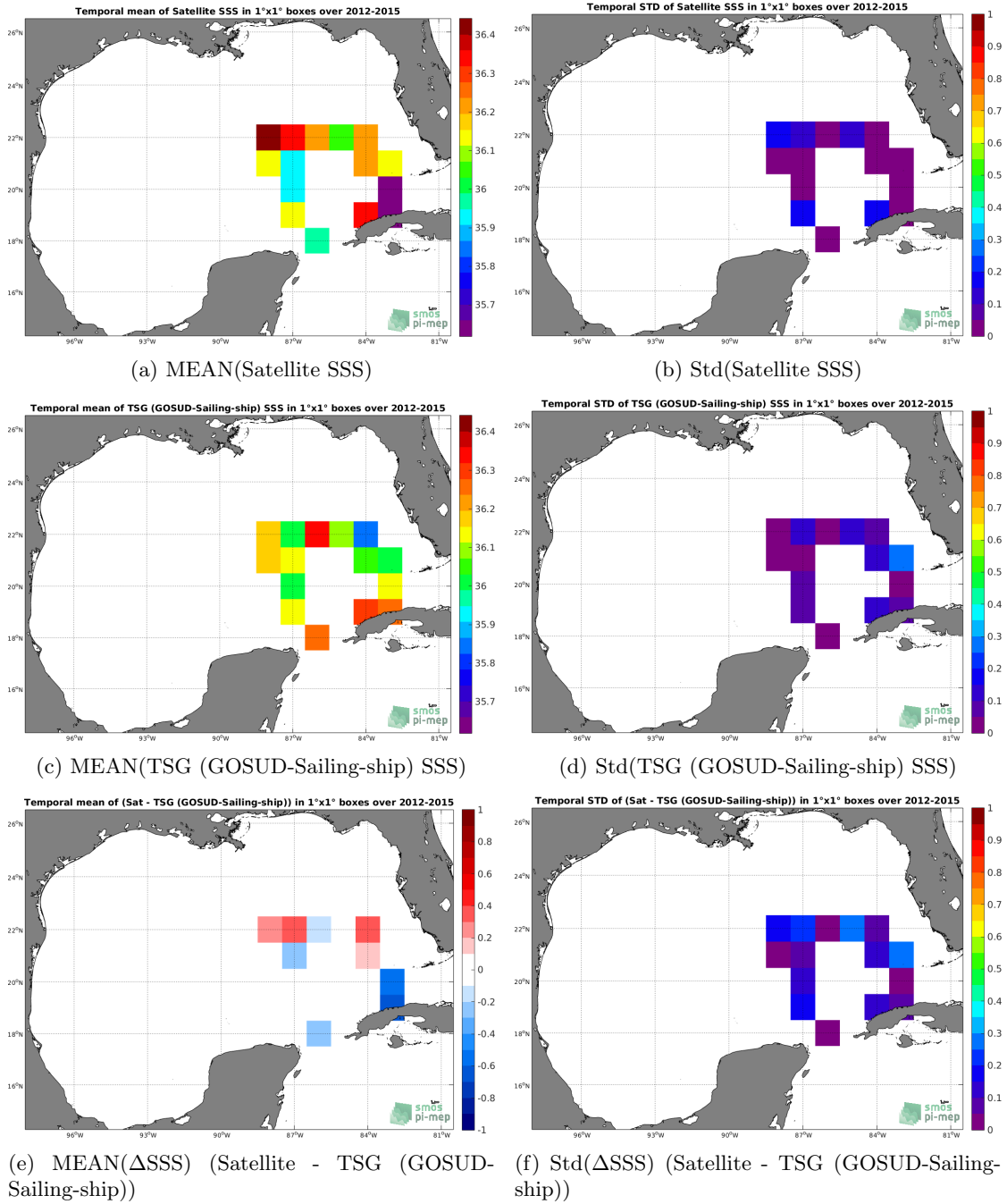
Figure 6: Temporal mean (left) and Std (right) of SSS from SMOS SSS L3 v2 - 9-Days (BEC) (top), TSG (GOSUD-Sailing-ship) (middle), and of \Delta SSS (Satellite - TSG (GOSUD-Sailing-ship)). Only match-up pairs are used to generate these maps.
