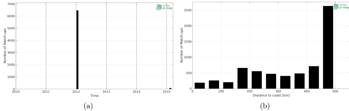
Figure 1: Number of match-ups between TSG (GOSUD-Sailing-ship) and SMOS SSS L3 v2 - 9-Days (BEC) SSS as a function of time (a) and as function of the distance to coast (b) over the Gulf of Mexico Pi-MEP region and for the full satellite product period.
