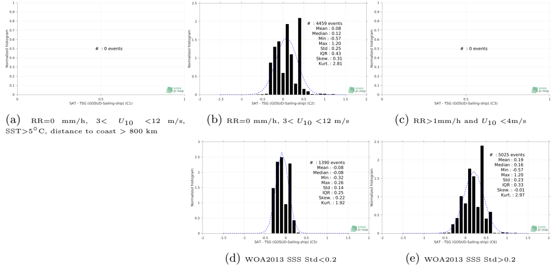
Figure 13: Normalized histogram of \Delta SSS (SMOS L3 v2 - 9-Days (BEC) - TSG (GOSUD-Sailing-ship)) for 5 different subdatasets corresponding to: RR=0 mm/h, 3 < U_{10} < 12 m/s, SST > 5^{\circ}C , distance to coast > 800 km (a), RR=0 mm/h, 3 < U_{10} < 12 m/s (b), RR > 1 mm/h and U_{10} < 4 m/s (c), WOA2013 SSS Std < 0.2 (d), WOA2013 SSS Std > 0.2 (e).
