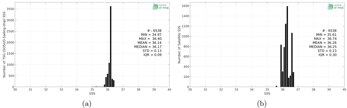
Figure 2: Histograms of SSS from TSG (GOSUD-Sailing-ship) (a) and SMOS L3 v2 - 9-Days (BEC) (b) considering all match-up pairs per bins of 0.1 over the Gulf of Mexico Pi-MEP region and for the full satellite product period.
