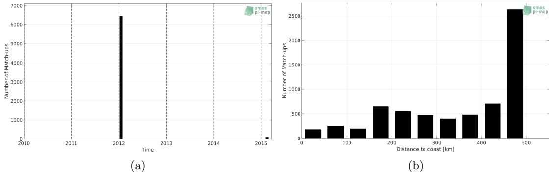
Figure 1: Number of match-ups between TSG (GOSUD-Sailing-ship) and SMOS L3 v2 - 9-Days (BEC) SSS as a function of time (a) and as function of the distance to coast (b) over the Gulf of Mexico Pi-MEP region and for the full satellite product period.
