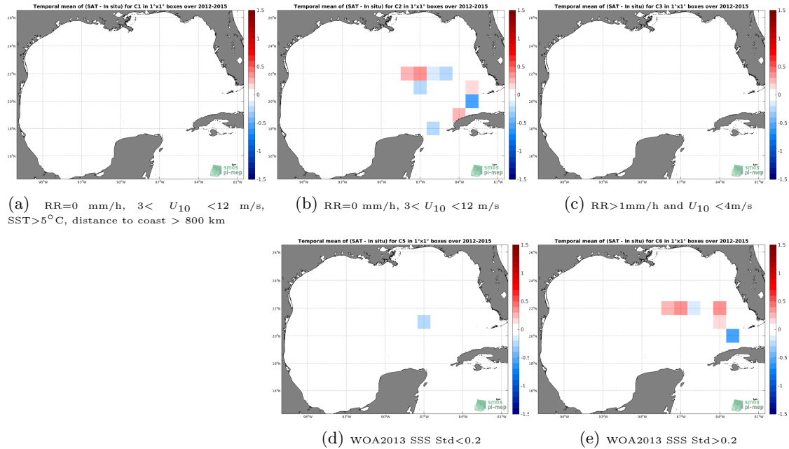
Figure 12: Temporal mean gridded over spatial boxes of size 1^\circ \times 1^\circ of \Delta SSS (SMOS L3 v2 - 9-Days (BEC) - TSG (GOSUD-Sailing-ship)) for 5 different subdatasets corresponding to:RR=0 mm/h, 3 < U_{10} < 12 m/s, SST >5^\circ\text{C} , distance to coast > 800 km (a), RR=0 mm/h, 3 < U_{10} < 12 m/s (b), RR >1 mm/h and U_{10} < 4 m/s (c), WOA2013 SSS Std <0.2 (d), WOA2013 SSS Std >0.2 (e).
