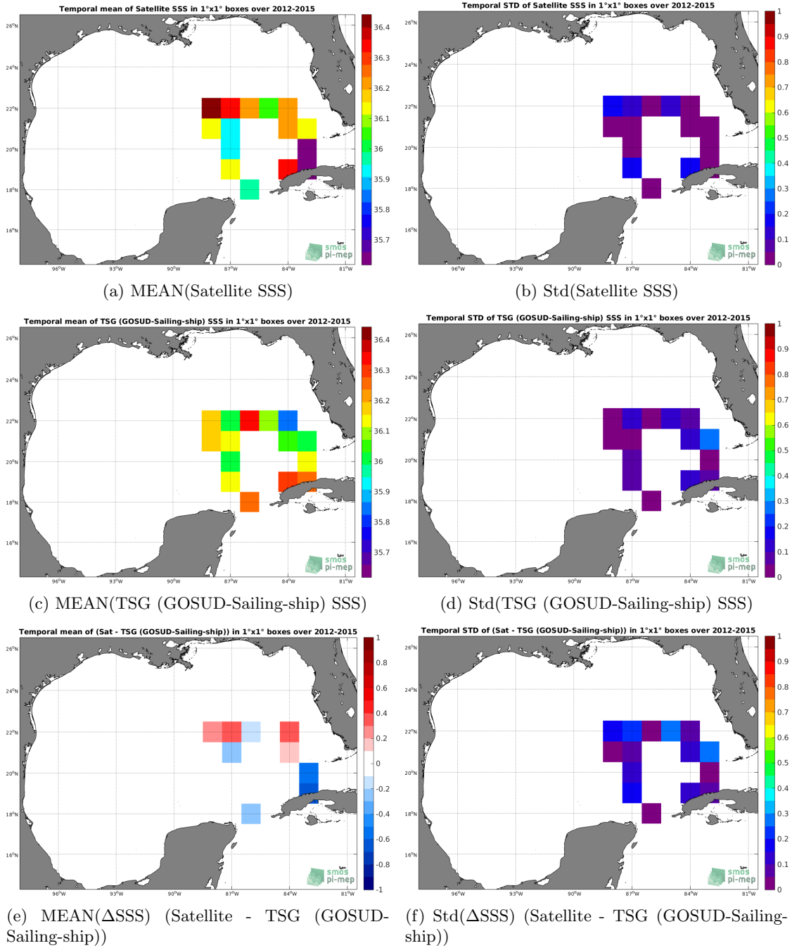
Figure 6: Temporal mean (left) and Std (right) of SSS from SMOS L3 v2 - 9-Days (BEC) (top), TSG (GOSUD-Sailing-ship) (middle), and of \Delta SSS (Satellite - TSG (GOSUD-Sailing-ship)). Only match-up pairs are used to generate these maps.
