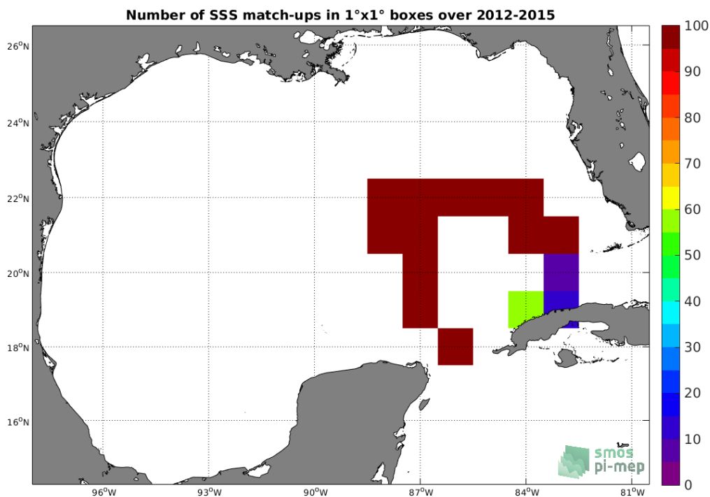
Figure 4: Number of SSS match-ups between TSG (GOSUD-Sailing-ship) SSS and the SMOS L3 v2 - 9-Days (BEC) SSS product for the Gulf of Mexico Pi-MEP region over 1^\circ \times 1^\circ boxes and for the full satellite product period.
