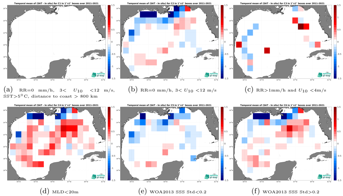
Figure 14: Temporal mean gridded over spatial boxes of size 1^\circ \times 1^\circ of \Delta SSS (SMOS SSS L3 v2 - 9-Days (BEC) - Argo) for 6 different subdatasets corresponding to: RR=0 mm/h, 3 < U_{10} < 12 m/s, SST > 5°C, distance to coast > 800 km (a), RR=0 mm/h, 3 < U_{10} < 12 m/s (b), RR > 1mm/h and U_{10} < 4 m/s (c), MLD < 20m (d), WOA2013 SSS Std < 0.2 (e), WOA2013 SSS Std > 0.2 (f).
