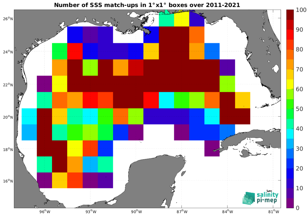
Figure 5: Number of SSS match-ups between Argo SSS and the SMOS SSS L3 v2 - 9-Days (BEC) SSS product for the Gulf of Mexico Pi-MEP region over 1^\circ \times 1^\circ boxes and for the full satellite product period.
