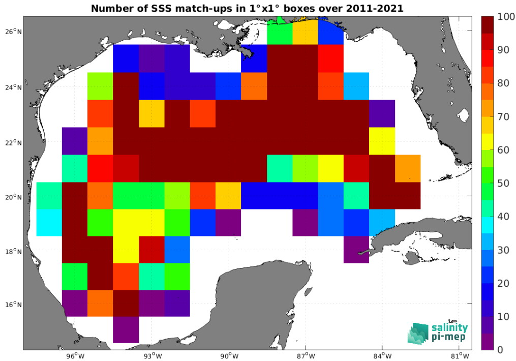
Figure 4: Number of SSS match-ups between Argo SSS and the SMOS SSS L3 v2 - 9-Days (BEC) SSS product for the Gulf of Mexico Pi-MEP region over 1^{\circ} \times 1^{\circ} boxes and for the full satellite product period.
