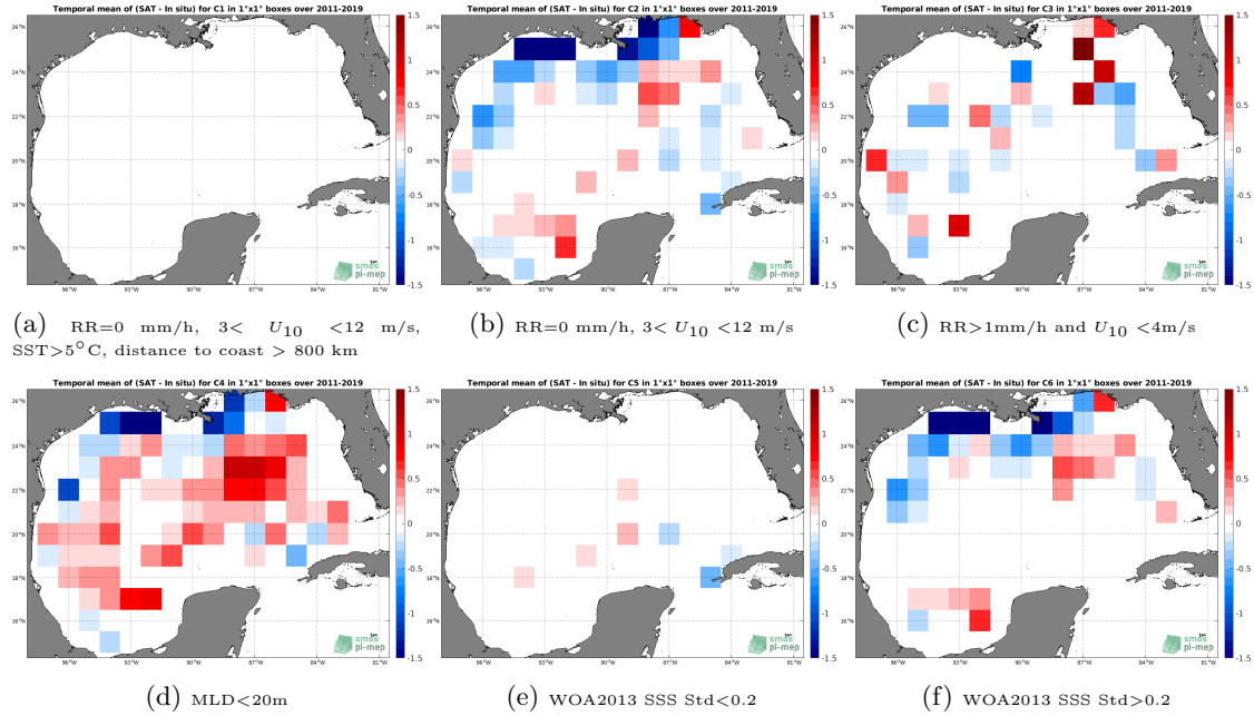
Figure 12: Temporal mean gridded over spatial boxes of size 1^\circ \times 1^\circ of \Delta SSS (SMOS SSS L3 v2 - 9-Days (BEC) - Argo) for 6 different subdatasets corresponding to:RR=0 mm/h, 3 < U_{10} < 12 m/s, SST >5^\circ\text{C} , distance to coast > 800 km (a), RR=0 mm/h, 3 < U_{10} < 12 m/s (b), RR >1 mm/h and U_{10} < 4 m/s (c),MLD <20 m (d),WOA2013 SSS Std <0.2 (e),WOA2013 SSS Std >0.2 (f).
