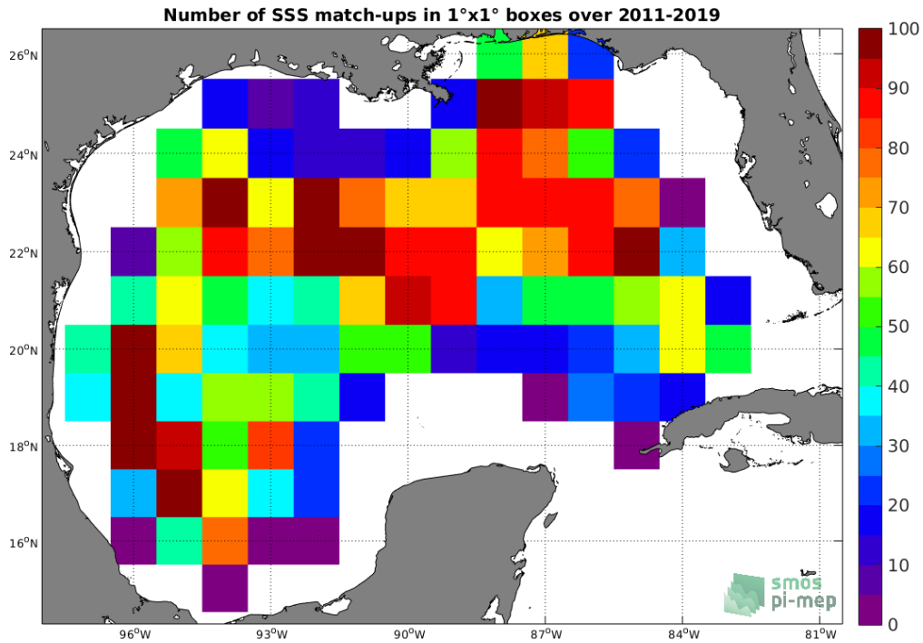
Figure 4: Number of SSS match-ups between Argo SSS and the SMOS L3 v2 - 9-Days (BEC) SSS product for the Gulf of Mexico Pi-MEP region over 1^\circ \times 1^\circ boxes and for the full satellite product period.
