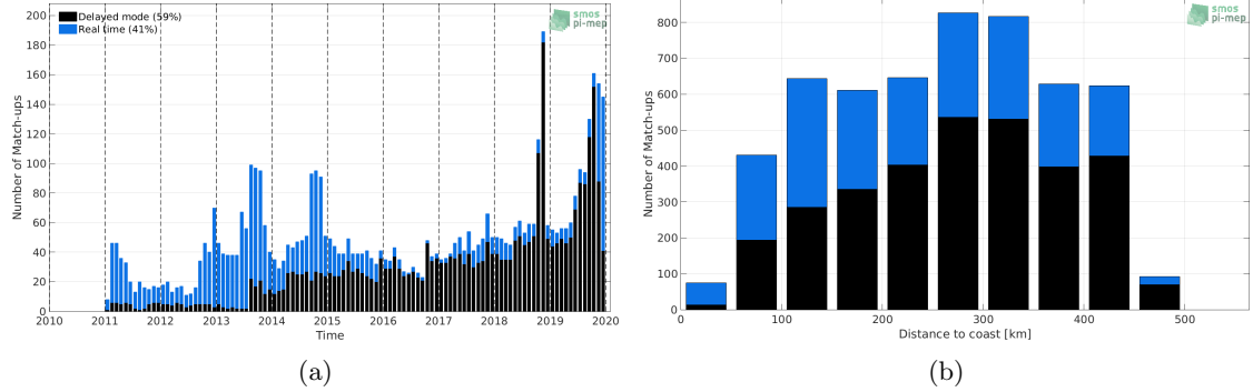
Figure 1: Number of match-ups between Argo and SMOS L3 v2 - 9-Days (BEC) SSS as a function of time (a) and as function of the distance to coast (b) over the Gulf of Mexico Pi-MEP region and for the full satellite product period.
