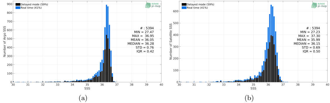
Figure 2: Histograms of SSS from Argo (a) and SMOS L3 v2 - 9-Days (BEC) (b) considering all match-up pairs per bins of 0.1 over the Gulf of Mexico Pi-MEP region and for the full satellite product period.
