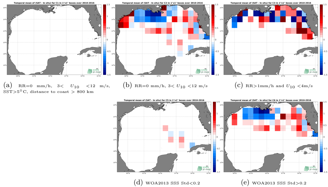
Figure 12: Temporal mean gridded over spatial boxes of size 1^\circ \times 1^\circ of \Delta SSS (SMOS-L3-BEC-OA-V1-9DAYS-0.25DEG - TSG-SAMOS) for 5 different subdatasets corresponding to:RR=0 mm/h, 3 < U_{10} < 12 m/s, SST >5^\circ C, distance to coast > 800 km (a), RR=0 mm/h, 3 < U_{10} < 12 m/s (b), RR >1 mm/h and U_{10} < 4 m/s (c), WOA2013 SSS Std <0.2 (d), WOA2013 SSS Std >0.2 (e).
