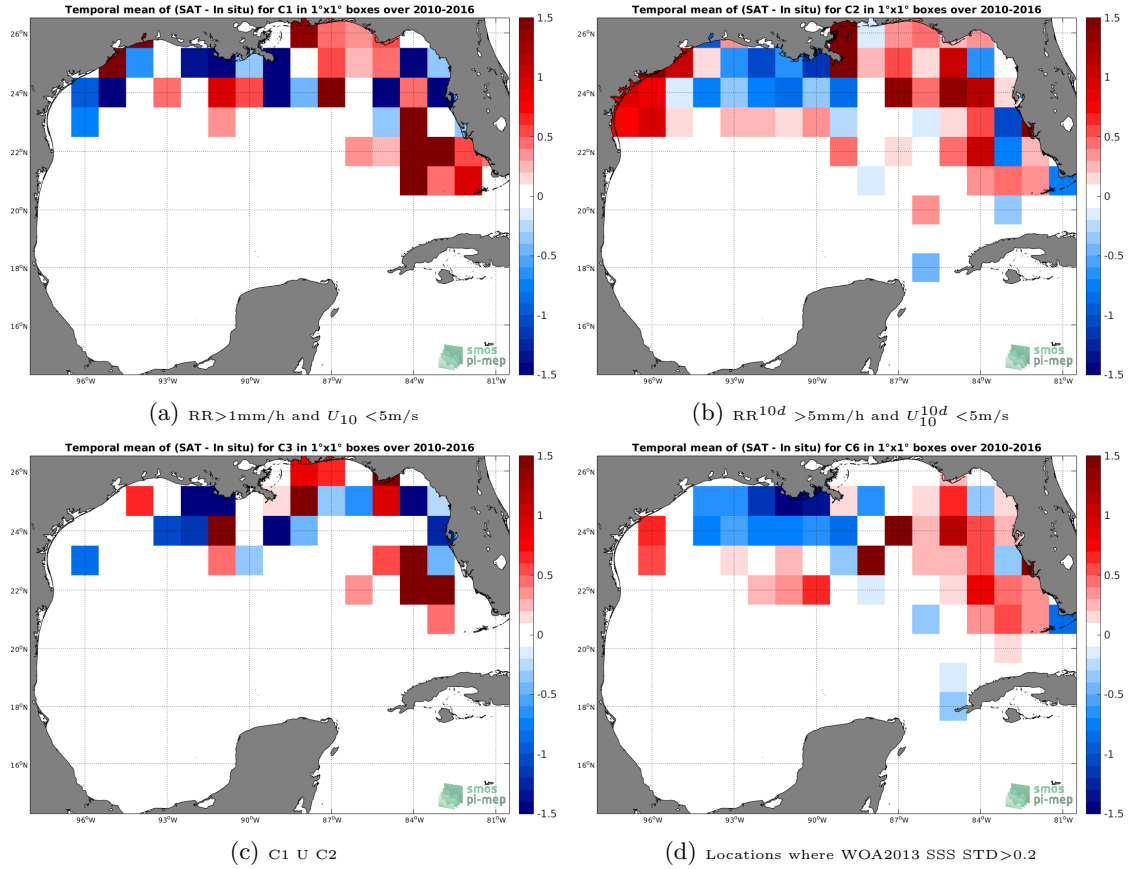
Figure 12: Temporal mean gridded over spatial boxes of size 1^\circ \times 1^\circ of \Delta SSS (SMOS-L3-BEC-OA-V1-9DAYS-0.25DEG - TSG-SAMOS) for 4 different subdatasets corresponding to:RR > 1\text{mm/h} and U_{10} < 5\text{m/s} (a), RR^{10d} > 5\text{mm/h} and U_{10}^{10d} < 5\text{m/s} (b), C1 U C2 (c),Locations where WOA2013 SSS STD > 0.2 (d).
