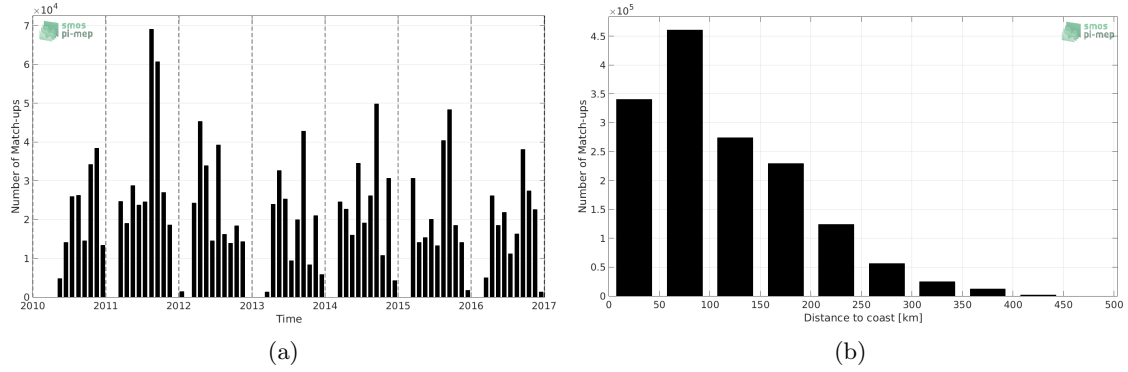
Figure 1: Number of match-ups between TSG-SAMOS and SMOS-L3-BEC-OA-V1-9DAYS-0.25DEG SSS as a function of time (a) and as function of the distance to coast (b) over the Gulf of Mexico Pi-MEP region and for the full satellite product period.
