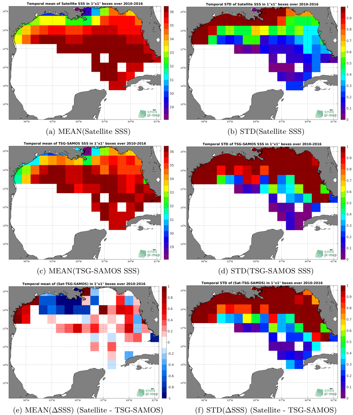
Figure 6: Temporal mean (left) and STD (right) of SSS from SMOS-L3-BEC-OA-V1-9DAYS-0.25DEG (top), TSG-SAMOS (middle), and of \Delta SSS (Satellite - TSG-SAMOS). Only match-up pairs are used to generate these maps.
