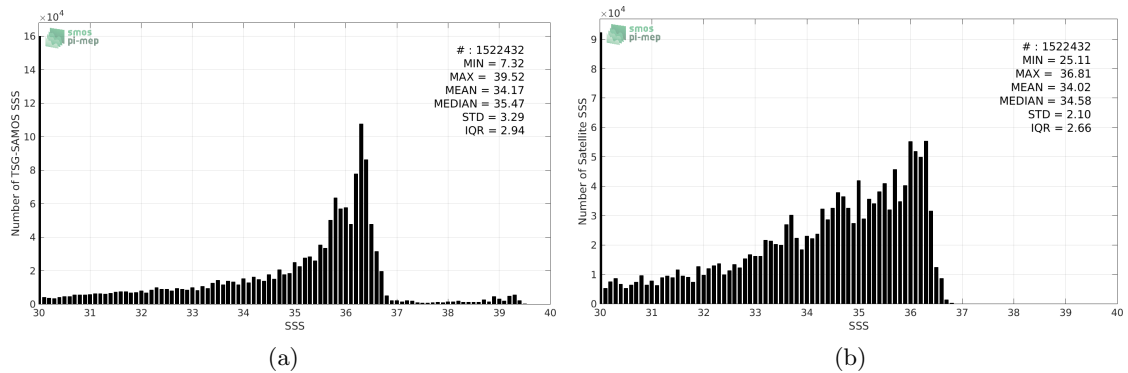
Figure 2: Histograms of SSS from TSG-SAMOS (a) and SMOS-L3-BEC-OA-V1-9DAYS-0.25DEG (b) considering all match-up pairs per bins of 0.1 over the Gulf of Mexico Pi-MEP region and for the full satellite product period.
