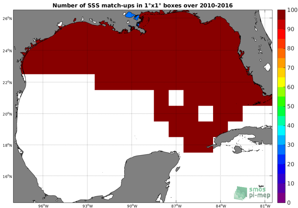
Figure 4: Number of SSS match-ups between TSG-SAMOS SSS and the SMOS-L3-BEC-OA-V1-9DAYS-0.25DEG SSS product for the Gulf of Mexico Pi-MEP region over 1^\circ \times 1^\circ boxes and for the full satellite product period.
