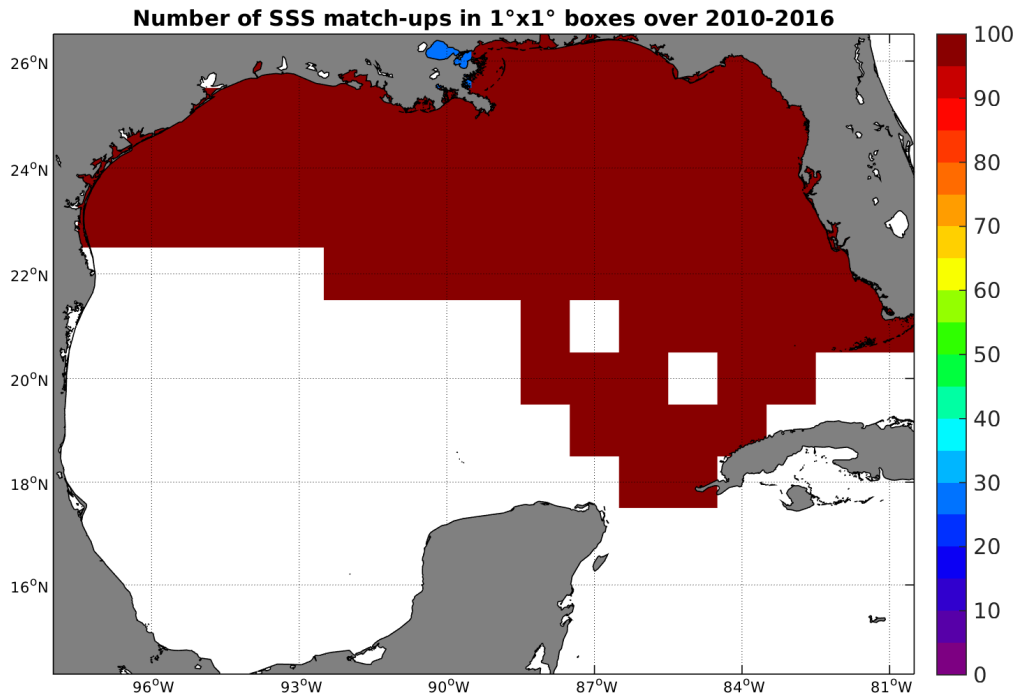
Figure 4: Number of SSS match-ups between TSG-SAMOS SSS and the SMOS-L3-BEC-OA-V1-9DAYS-0.25DEG SSS product for the Gulf of Mexico Pi-MEP region over 1^\circ \times 1^\circ boxes and for the full satellite product period.
