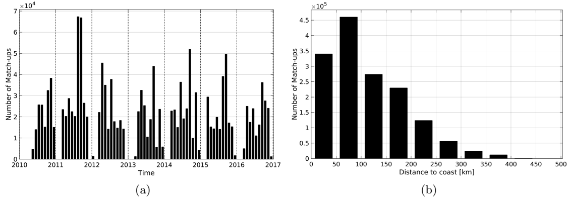
Figure 1: Number of match-ups between TSG-SAMOS and SMOS-L3-BEC-OA-V1-9DAYS-0.25DEG SSS as a function of time (a) and as function of the distance to coast (b) over the Gulf of Mexico Pi-MEP region and for the full satellite product period.
