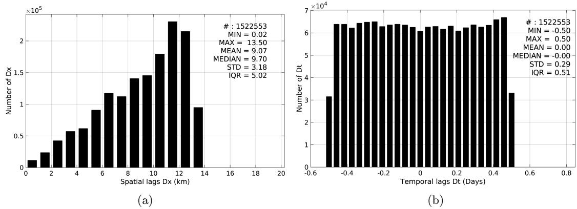
Figure 5: Histograms of the spatial (a) and temporal (b) lags between the time of the TSG-SAMOS measurements and the date of the corresponding SMOS-L3-BEC-OA-V1-9DAYS-0.25DEG SSS product.
