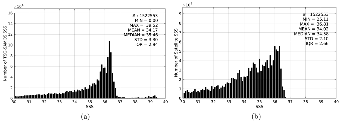
Figure 2: Histograms of SSS from TSG-SAMOS (a) and SMOS-L3-BEC-OA-V1-9DAYS-0.25DEG (b) considering all match-up pairs per bins of 0.1 over the Gulf of Mexico Pi-MEP region and for the full satellite product period.
