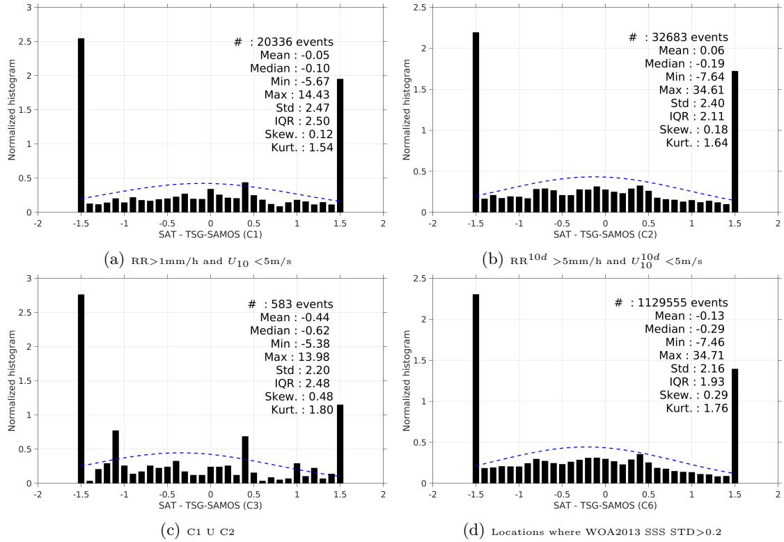
Figure 13: Normalized histogram of \Delta\text{SSS} (SMOS-L3-BEC-OA-V1-9DAYS-0.25DEG - TSG-SAMOS) for 6 different subdatasets corresponding to: \text{RR} > 1\text{mm/h} and U_{10} < 5\text{m/s} (a), \text{RR}^{10d} > 5\text{mm/h} and U_{10}^{10d} < 5\text{m/s} (b), C1 U C2 (c), Locations where WOA2013 SSS STD > 0.2 (d).
