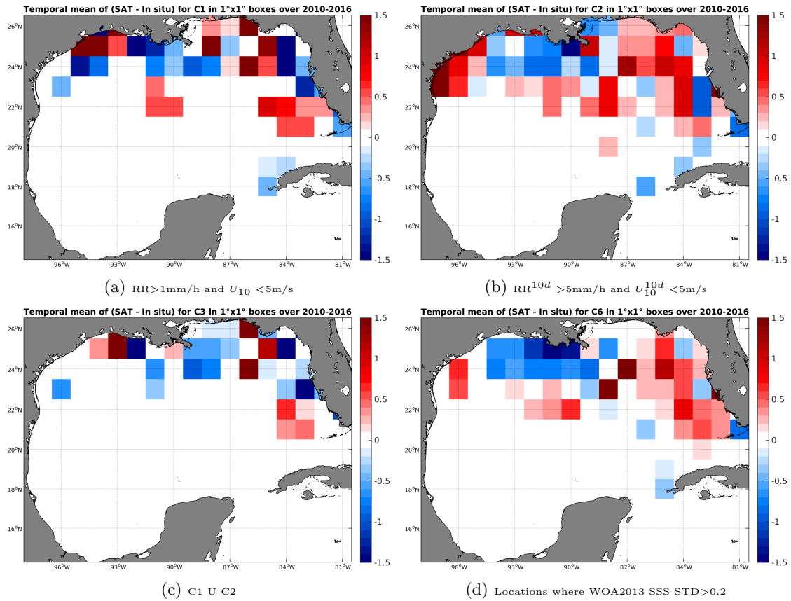
Figure 12: Temporal mean gridded over spatial boxes of size 1^\circ \times 1^\circ of \Delta SSS (SMOS-L3-BEC-OA-V1-9DAYS-0.25DEG - TSG-SAMOS) for 4 different subdatasets corresponding to:RR > 1mm/h and U_{10} < 5 m/s (a), RR^{10d} > 5 mm/h and U_{10}^{10d} < 5 m/s (b), C1 U C2 (c),Locations where WOA2013 SSS STD > 0.2 (d).
