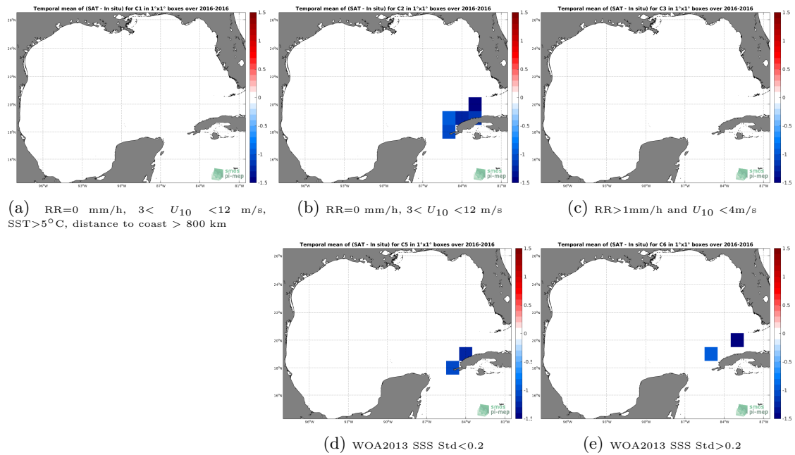
Figure 12: Temporal mean gridded over spatial boxes of size 1^\circ \times 1^\circ of \Delta SSS (SMOS-L3-BEC-OA-V1-9DAYS-0.25DEG - TSG-LEGOS-DM) for 5 different subdatasets corresponding to: RR=0 mm/h, 3 < U_{10} < 12 m/s, SST > 5^\circ\text{C} , distance to coast > 800 km (a), RR=0 mm/h, 3 < U_{10} < 12 m/s (b), RR > 1 mm/h and U_{10} < 4 m/s (c), WOA2013 SSS Std < 0.2 (d), WOA2013 SSS Std > 0.2 (e).
