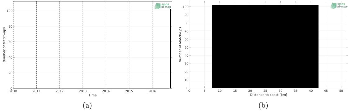
Figure 1: Number of match-ups between TSG-LEGOS-DM and SMOS-L3-BEC-OA-V1-9DAYS-0.25DEG SSS as a function of time (a) and as function of the distance to coast (b) over the Gulf of Mexico Pi-MEP region and for the full satellite product period.
