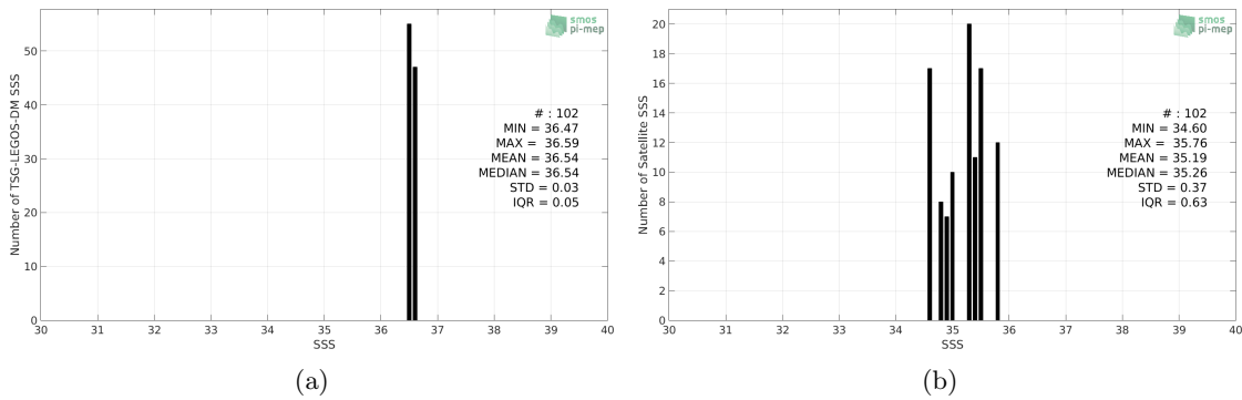
Figure 2: Histograms of SSS from TSG-LEGOS-DM (a) and SMOS-L3-BEC-OA-V1-9DAYS-0.25DEG (b) considering all match-up pairs per bins of 0.1 over the Gulf of Mexico Pi-MEP region and for the full satellite product period.
