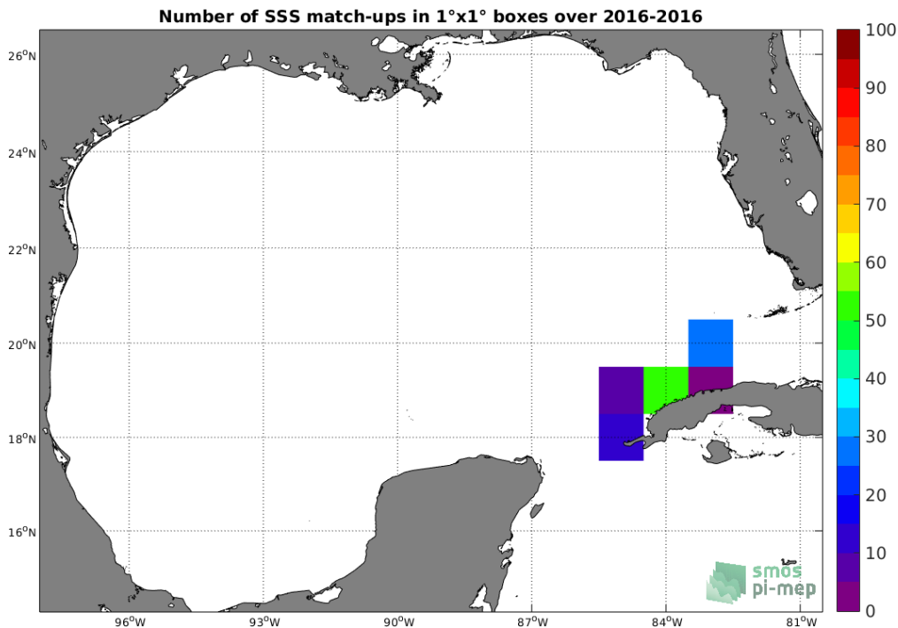
Figure 4: Number of SSS match-ups between TSG-LEGOS-DM SSS and the SMOS-L3-BEC-OA-V1-9DAYS-0.25DEG SSS product for the Gulf of Mexico Pi-MEP region over 1°x1° boxes and for the full satellite product period.
