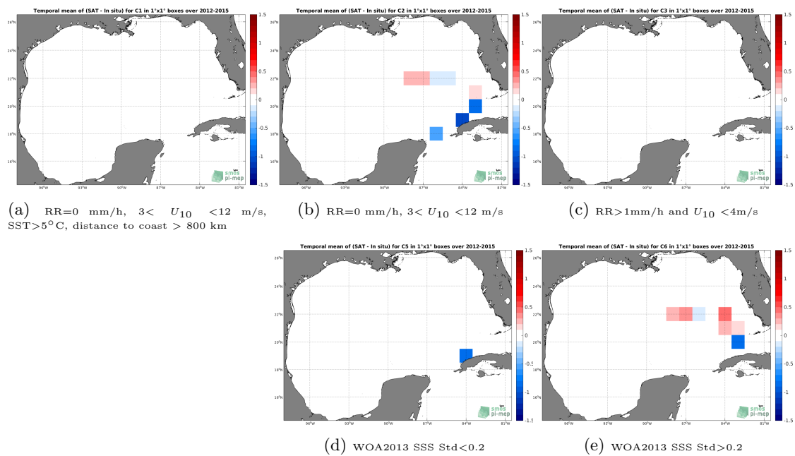
Figure 12: Temporal mean gridded over spatial boxes of size 1^\circ \times 1^\circ of \Delta SSS (SMOS-L3-BEC-OA-V1-9DAYS-0.25DEG - TSG-GOSUD-Sailing-ship) for 5 different subdatasets corresponding to:RR=0 mm/h, 3 < U_{10} < 12 m/s, SST>5°C, distance to coast > 800 km (a), RR=0 mm/h, 3 < U_{10} < 12 m/s (b), RR>1mm/h and U_{10} < 4 m/s (c), WOA2013 SSS Std<0.2 (d), WOA2013 SSS Std>0.2 (e).
