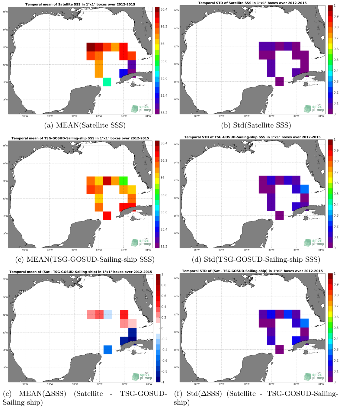
Figure 6: Temporal mean (left) and Std (right) of SSS from SMOS-L3-BEC-OA-V1-9DAYS-0.25DEG (top), TSG-GOSUD-Sailing-ship (middle), and of \Delta SSS (Satellite - TSG-GOSUD-Sailing-ship). Only match-up pairs are used to generate these maps.
