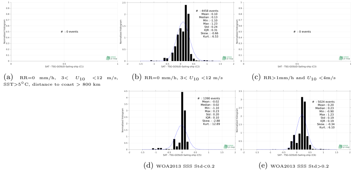
Figure 13: Normalized histogram of \Delta SSS (SMOS-L3-BEC-OA-V1-9DAYS-0.25DEG - TSG-GOSUD-Sailing-ship) for 5 different subdatasets corresponding to: RR=0 mm/h, 3 < U_{10} < 12 m/s, SST > 5°C, distance to coast > 800 km (a), RR=0 mm/h, 3 < U_{10} < 12 m/s (b), RR > 1mm/h and U_{10} < 4 m/s (c), WOA2013 SSS Std < 0.2 (d), WOA2013 SSS Std > 0.2 (e).
