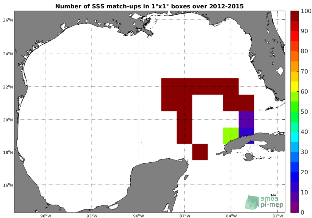
Figure 4: Number of SSS match-ups between TSG-GOSUD-Sailing-ship SSS and the SMOS-L3-BEC-OA-V1-9DAYS-0.25DEG SSS product for the Gulf of Mexico Pi-MEP region over 1^\circ \times 1^\circ boxes and for the full satellite product period.
