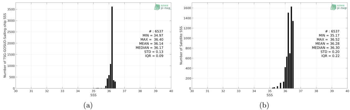
Figure 2: Histograms of SSS from TSG-GOSUD-Sailing-ship (a) and SMOS-L3-BEC-OA-V1-9DAYS-0.25DEG (b) considering all match-up pairs per bins of 0.1 over the Gulf of Mexico Pi-MEP region and for the full satellite product period.
