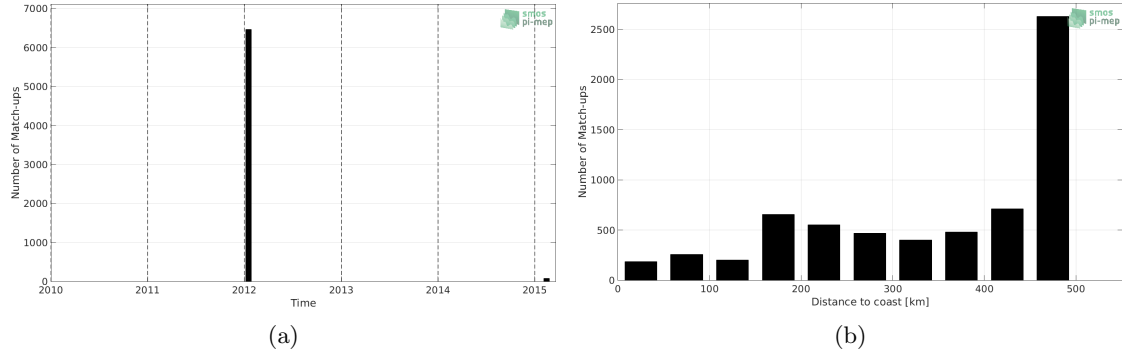
Figure 1: Number of match-ups between TSG-GOSUD-Sailing-ship and SMOS-L3-BEC-OA-V1-9DAYS-0.25DEG SSS as a function of time (a) and as function of the distance to coast (b) over the Gulf of Mexico Pi-MEP region and for the full satellite product period.
