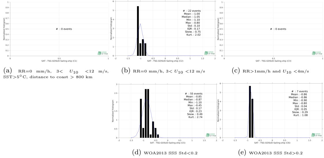
Figure 13: Normalized histogram of \Delta SSS (SMOS-L3-BEC-OA-V1-9DAYS-0.25DEG - TSG-GOSUD-Sailing-ship) for 5 different subdatasets corresponding to: RR=0 mm/h, 3 < U_{10} < 12 m/s, SST > 5^\circ\text{C} , distance to coast > 800 km (a), RR=0 mm/h, 3 < U_{10} < 12 m/s (b), RR > 1\text{mm/h} and U_{10} < 4\text{m/s} (c), WOA2013 SSS Std < 0.2 (d), WOA2013 SSS Std > 0.2 (e).
