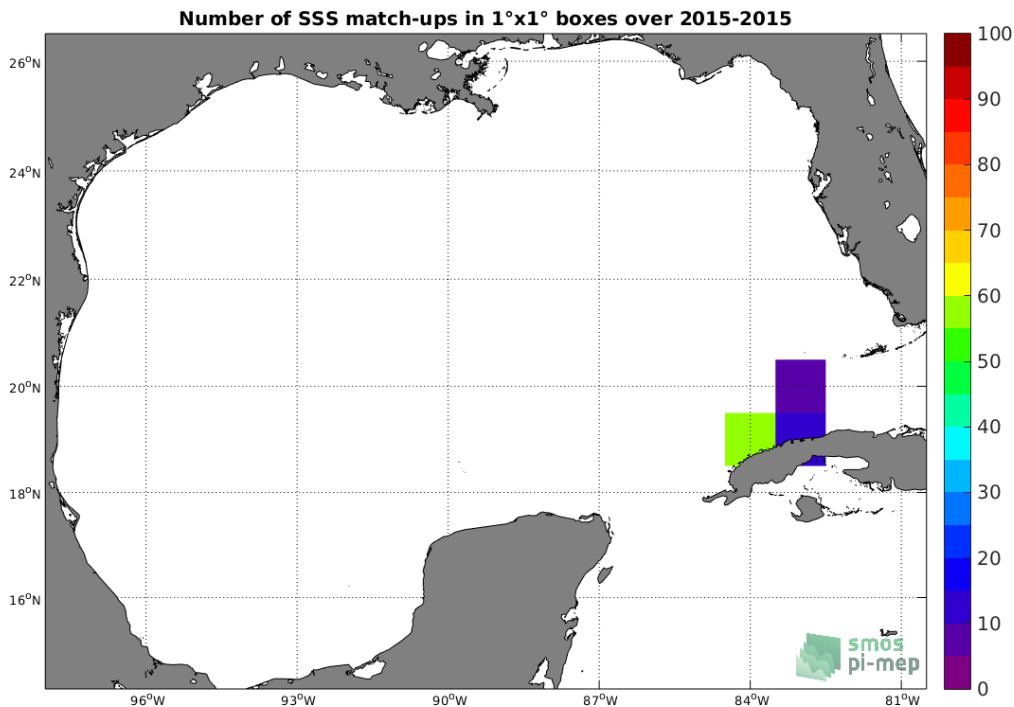
Figure 4: Number of SSS match-ups between TSG-GOSUD-Sailing-ship SSS and the SMOS-L3-BEC-OA-V1-9DAYS-0.25DEG SSS product for the Gulf of Mexico Pi-MEP region over 1°x1° boxes and for the full satellite product period.
