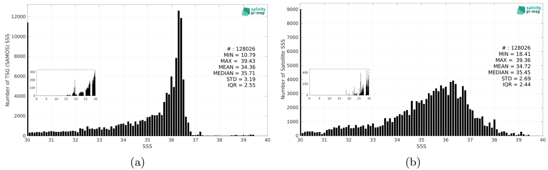
Figure 3: Histograms of SSS from TSG (SAMOS) (a) and SMOS SSS L2 v700 (ESA) (b) considering all match-up pairs per bins of 0.1 over the Gulf of Mexico Pi-MEP region and for the full satellite product period.
