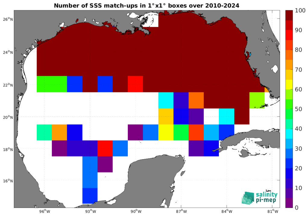
Figure 5: Number of SSS match-ups between TSG (SAMOS) SSS and the SMOS SSS L2 v700 (ESA) SSS product for the Gulf of Mexico Pi-MEP region over 1^\circ \times 1^\circ boxes and for the full satellite product period.
