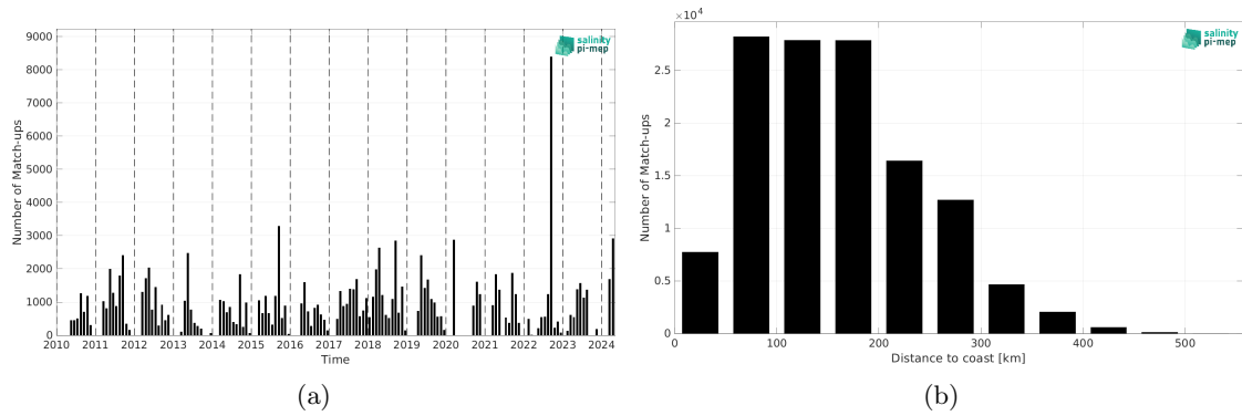
Figure 2: Number of match-ups between TSG (SAMOS) and SMOS SSS L2 v700 (ESA) SSS as a function of time (a) and as function of the distance to coast (b) over the Gulf of Mexico Pi-MEP region and for the full satellite product period.
