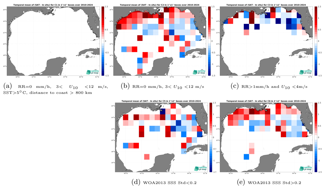
Figure 14: Temporal mean gridded over spatial boxes of size 1^\circ \times 1^\circ of \Delta SSS (SMOS SSS L2 v700 (ESA) - TSG (SAMOS)) for 5 different subdatasets corresponding to:RR=0 mm/h, 3 < U_{10} < 12 m/s, SST >5^\circ\text{C} , distance to coast > 800 km (a), RR=0 mm/h, 3 < U_{10} < 12 m/s (b), RR >1 mm/h and U_{10} < 4 m/s (c), WOA2013 SSS Std <0.2 (d), WOA2013 SSS Std >0.2 (e).
