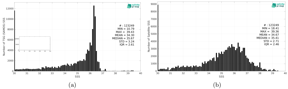
Figure 2: Histograms of SSS from TSG (SAMOS) (a) and SMOS SSS L2 v700 (ESA) (b) considering all match-up pairs per bins of 0.1 over the Gulf of Mexico Pi-MEP region and for the full satellite product period.
