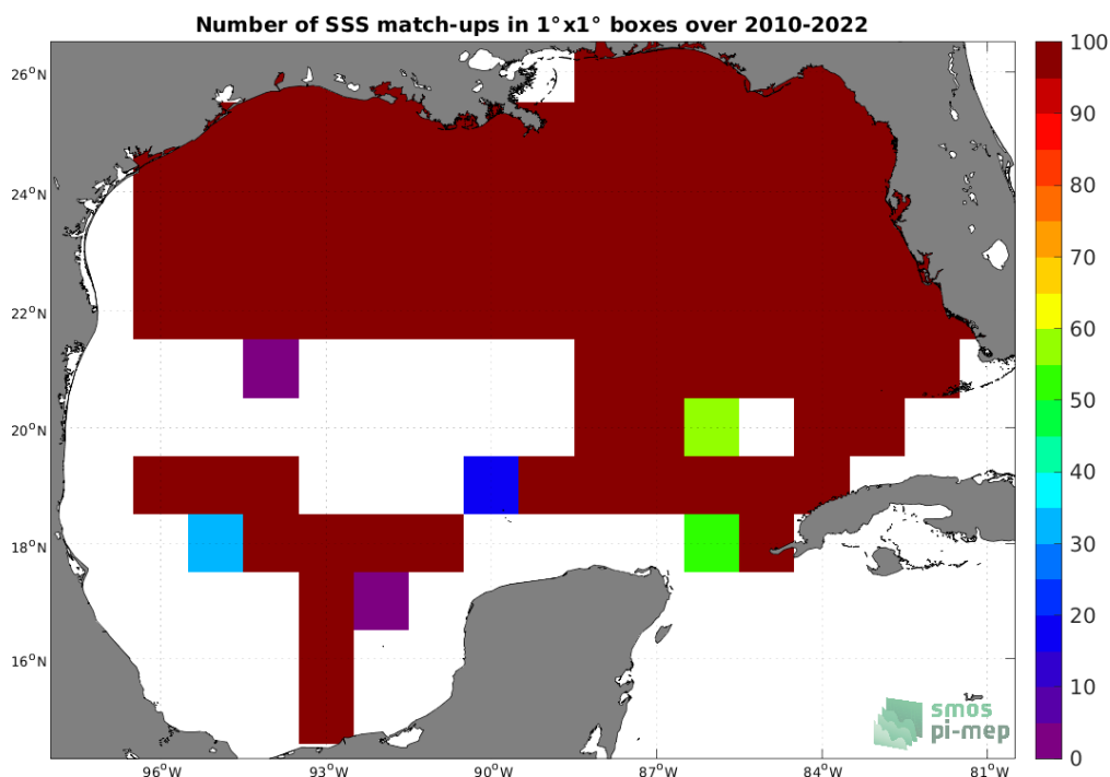
Figure 4: Number of SSS match-ups between TSG (SAMOS) SSS and the SMOS SSS L2 v700 (ESA) SSS product for the Gulf of Mexico Pi-MEP region over 1^{\circ} \times 1^{\circ} boxes and for the full satellite product period.
