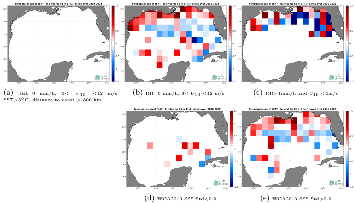
Figure 12: Temporal mean gridded over spatial boxes of size 1^\circ \times 1^\circ of \Delta SSS (SMOS SSS L2 v700 (ESA) - TSG (SAMOS)) for 5 different subdatasets corresponding to:RR=0 mm/h, 3 < U_{10} < 12 m/s, SST >5^\circ C, distance to coast > 800 km (a), RR=0 mm/h, 3 < U_{10} < 12 m/s (b), RR >1 mm/h and U_{10} < 4 m/s (c), WOA2013 SSS Std <0.2 (d), WOA2013 SSS Std >0.2 (e).
