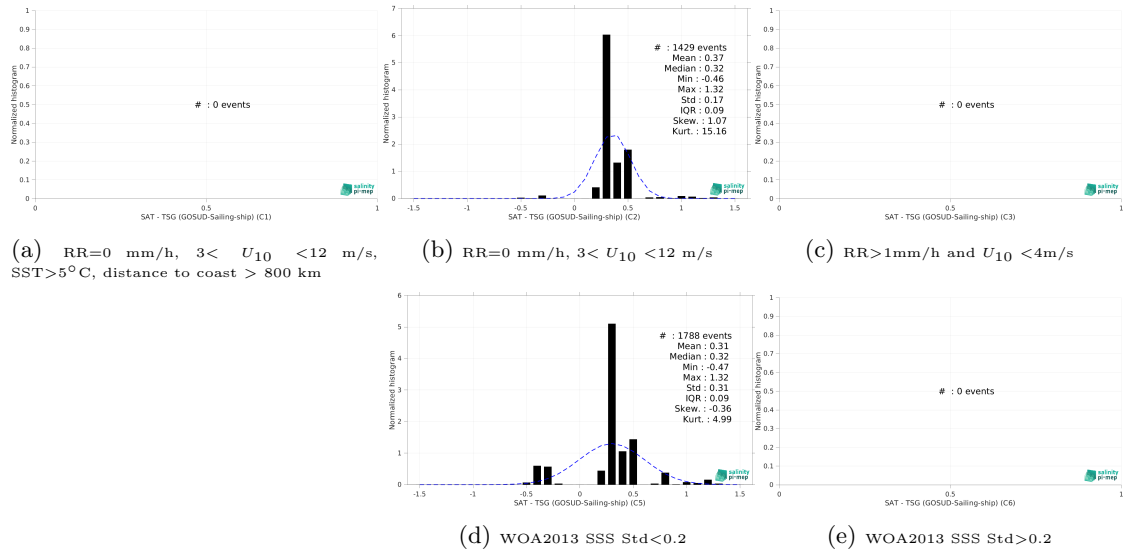
Figure 15: Normalized histogram of \Delta\text{SSS} (SMOS SSS L2 v700 (ESA) - TSG (GOSUD-Sailing-ship)) for 5 different subdatasets corresponding to: RR=0 mm/h, 3 < U_{10} < 12 m/s, SST > 5^\circ\text{C} , distance to coast > 800 km (a), RR=0 mm/h, 3 < U_{10} < 12 m/s (b), RR > 1\text{mm/h} and U_{10} < 4\text{m/s} (c), WOA2013 SSS Std < 0.2 (d), WOA2013 SSS Std > 0.2 (e).
