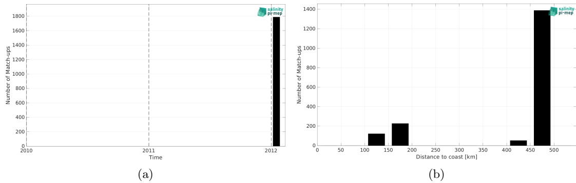
Figure 2: Number of match-ups between TSG (GOSUD-Sailing-ship) and SMOS SSS L2 v700 (ESA) SSS as a function of time (a) and as function of the distance to coast (b) over the Gulf of Mexico Pi-MEP region and for the full satellite product period.
