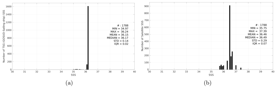
Figure 3: Histograms of SSS from TSG (GOSUD-Sailing-ship) (a) and SMOS SSS L2 v700 (ESA) (b) considering all match-up pairs per bins of 0.1 over the Gulf of Mexico Pi-MEP region and for the full satellite product period.
