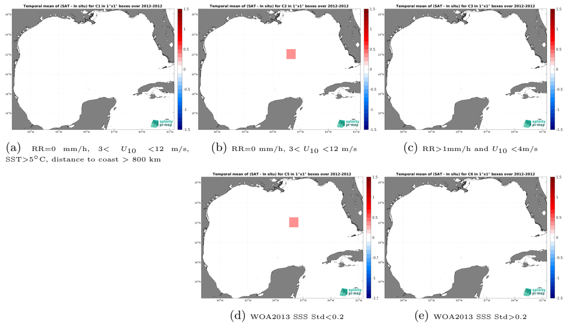
Figure 12: Temporal mean gridded over spatial boxes of size 1^\circ \times 1^\circ of \Delta SSS (SMOS SSS L2 v700 (ESA) - TSG (GOSUD-Sailing-ship)) for 5 different subdatasets corresponding to:RR=0 mm/h, 3 < U_{10} < 12 m/s, SST >5^\circ\text{C} , distance to coast > 800 km (a), RR=0 mm/h, 3 < U_{10} < 12 m/s (b), RR >1 mm/h and U_{10} < 4 m/s (c), WOA2013 SSS Std <0.2 (d), WOA2013 SSS Std >0.2 (e).
