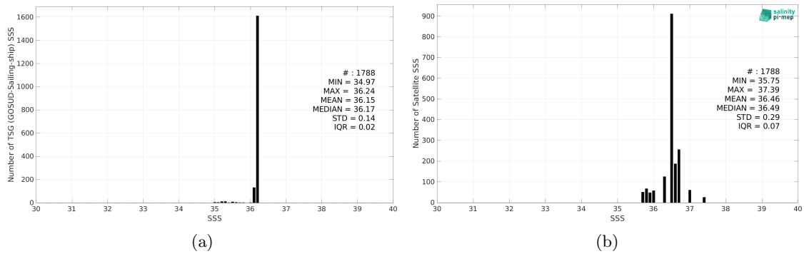
Figure 2: Histograms of SSS from TSG (GOSUD-Sailing-ship) (a) and SMOS SSS L2 v700 (ESA) (b) considering all match-up pairs per bins of 0.1 over the Gulf of Mexico Pi-MEP region and for the full satellite product period.
