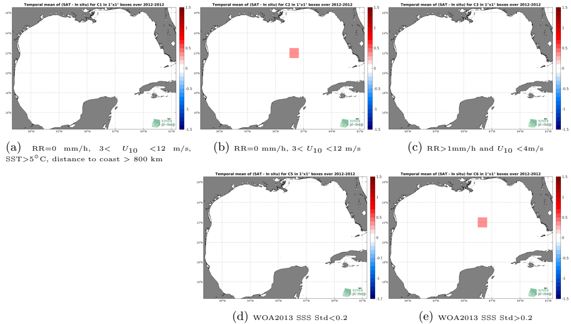
Figure 12: Temporal mean gridded over spatial boxes of size 1^{\circ}\times 1^{\circ} of \Delta SSS (SMOS SSS L2 v700 (ESA) - TSG (GOSUD-Sailing-ship)) for 5 different subdatasets corresponding to:RR=0 mm/h, 3 < U_{10} < 12 m/s, SST >5^{\circ}\text{C} , distance to coast > 800 km (a), RR=0 mm/h, 3 < U_{10} < 12 m/s (b), RR >1 mm/h and U_{10} < 4 m/s (c), WOA2013 SSS Std <0.2 (d), WOA2013 SSS Std >0.2 (e).
