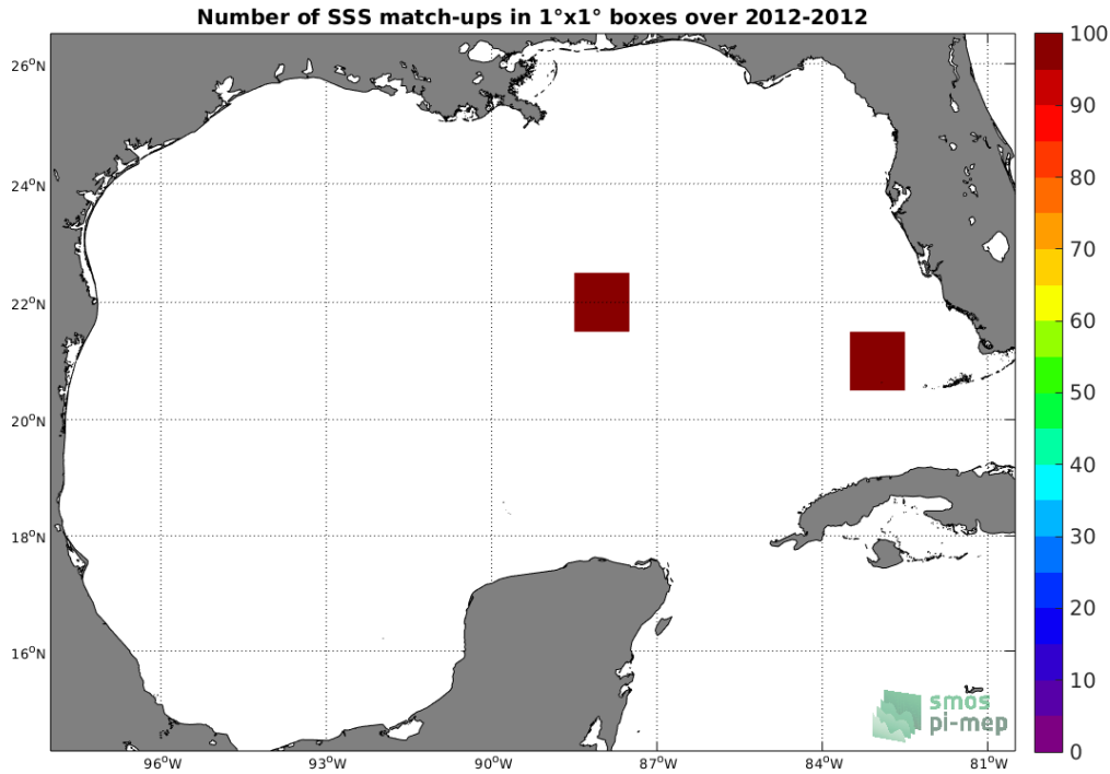
Figure 4: Number of SSS match-ups between TSG (GOSUD-Sailing-ship) SSS and the SMOS SSS L2 v700 (ESA) SSS product for the Gulf of Mexico Pi-MEP region over 1°x1° boxes and for the full satellite product period.
