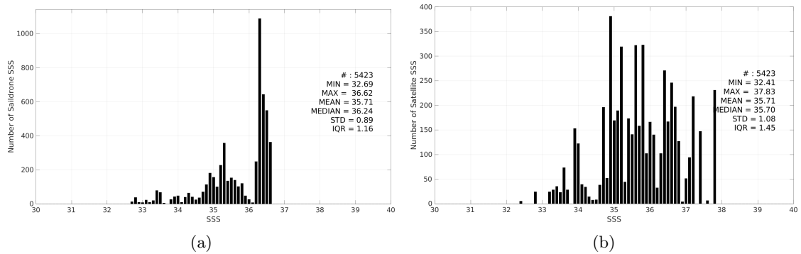
Figure 3: Histograms of SSS from Sairdrone (a) and SMOS SSS L2 v700 (ESA) (b) considering all match-up pairs per bins of 0.1 over the Gulf of Mexico Pi-MEP region and for the full satellite product period.
