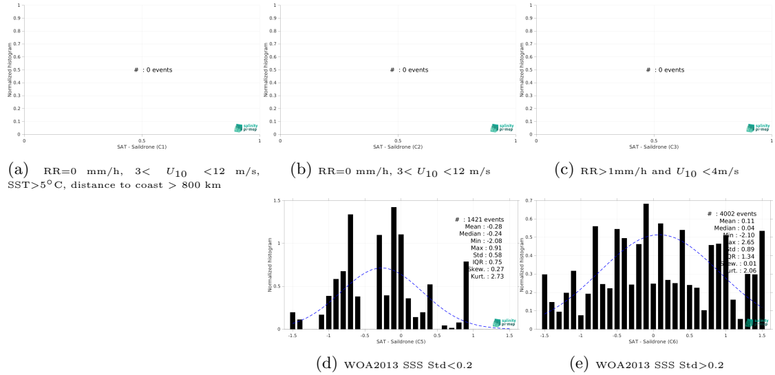
Figure 15: Normalized histogram of \Delta\text{SSS} (SMOS SSS L2 v700 (ESA) - Saiclone) for 5 different subdatasets corresponding to: RR=0 mm/h, 3 < U_{10} < 12 m/s, SST>5°C, distance to coast > 800 km (a), RR=0 mm/h, 3 < U_{10} < 12 m/s (b), RR>1mm/h and U_{10} < 4 m/s (c), WOA2013 SSS Std<0.2 (d), WOA2013 SSS Std>0.2 (e).
