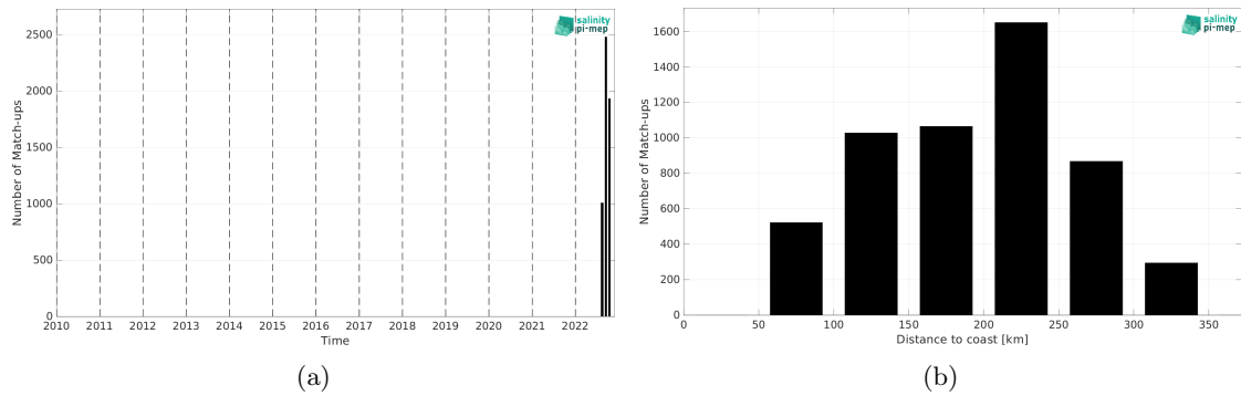
Figure 2: Number of match-ups between Sairdrone and SMOS SSS L2 v700 (ESA) SSS as a function of time (a) and as function of the distance to coast (b) over the Gulf of Mexico Pi-MEP region and for the full satellite product period.
