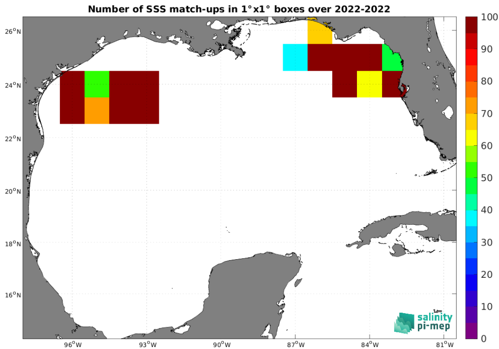
Figure 5: Number of SSS match-ups between Saildrone SSS and the SMOS SSS L2 v700 (ESA) SSS product for the Gulf of Mexico Pi-MEP region over 1°×1° boxes and for the full satellite product period.
