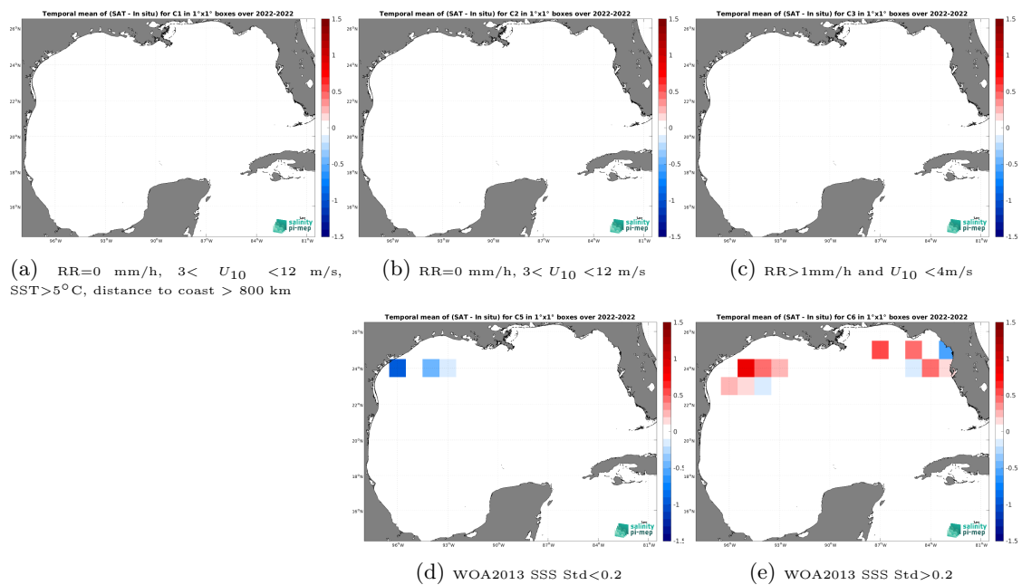
Figure 14: Temporal mean gridded over spatial boxes of size 1^\circ \times 1^\circ of \Delta SSS (SMOS SSS L2 v700 (ESA) - Saildrone) for 5 different subdatasets corresponding to:RR=0 mm/h, 3 < U_{10} < 12 m/s, SST >5^\circ\text{C} , distance to coast > 800 km (a), RR=0 mm/h, 3 < U_{10} < 12 m/s (b), RR >1 mm/h and U_{10} < 4 m/s (c), WOA2013 SSS Std <0.2 (d), WOA2013 SSS Std >0.2 (e).
